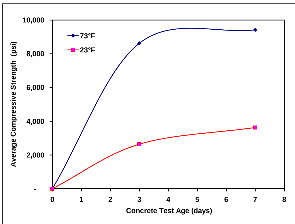
Figure 11. Early age strength development for Mixture 10 at ambient and 23 °F.
