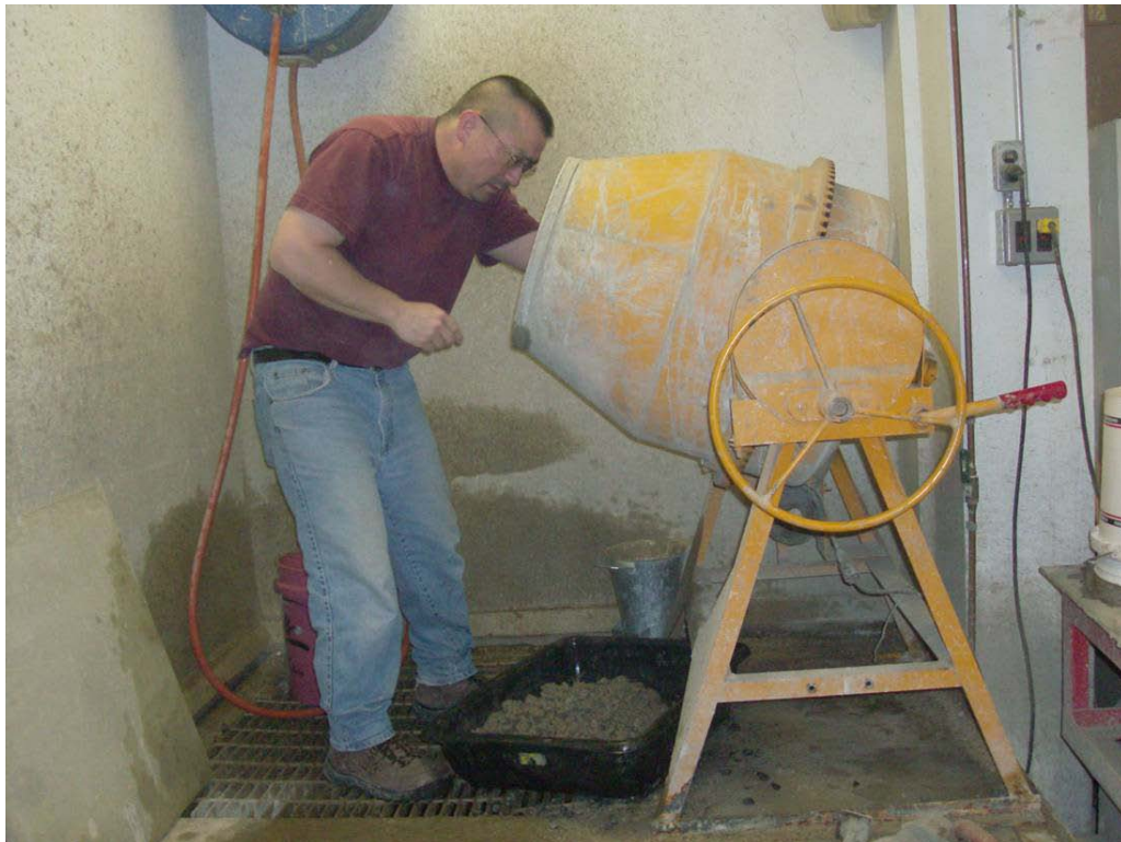
Figure 2. Laboratory mixer setup.
