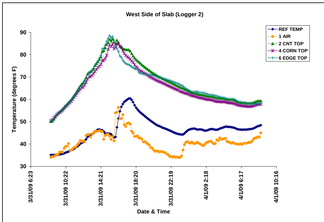
Figure 33. Temperature readings for the near surface at the center, corner, and edge at the western edge.
