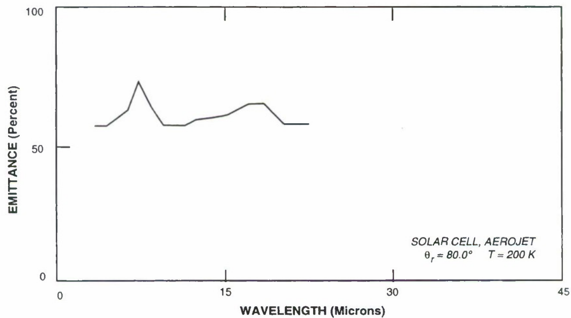
Figure 7. Emissivity vs. wavelength for silicon solar cells.
