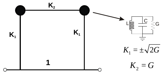
Fig. 4. Generalized coupled-resonator model of a matched notch filter.
