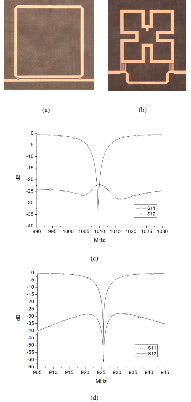
Fig. 6. Dual-mode notch filters: (a) microstrip ring-resonator prototype ( 56 \times 56\ \text{mm}^2 ) (b) microstrip folded-ring resonator prototype ( 40 \times 40\ \text{mm}^2 ) (c) ring-resonator measured results (d) folded-ring resonator measured results.
