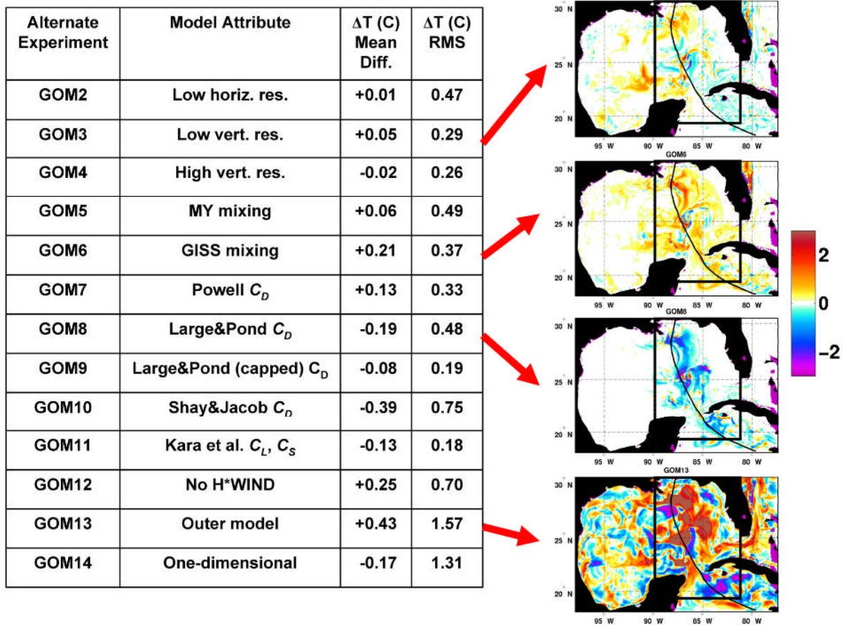
Figure 7. Sensitivity analysis of SST change forced by hurricane Ivan (track in black line), as summarized by differences in the SST change (Sept. 17 minus Sept. 11) calculated using Equation (2) between the control experiment GOM1 and each of the remaining experiments GOM2-GOM14. The RMS amplitude of \Delta T (°C), which represents the RMS difference between the SST changes forced by the two experiments, are tabulated in the third column. Four \Delta T maps are shown as examples. All RMS \Delta T values are calculated within the rectangular boxes outlined by black lines in the maps (extreme NW Caribbean Sea and eastern GoM).
