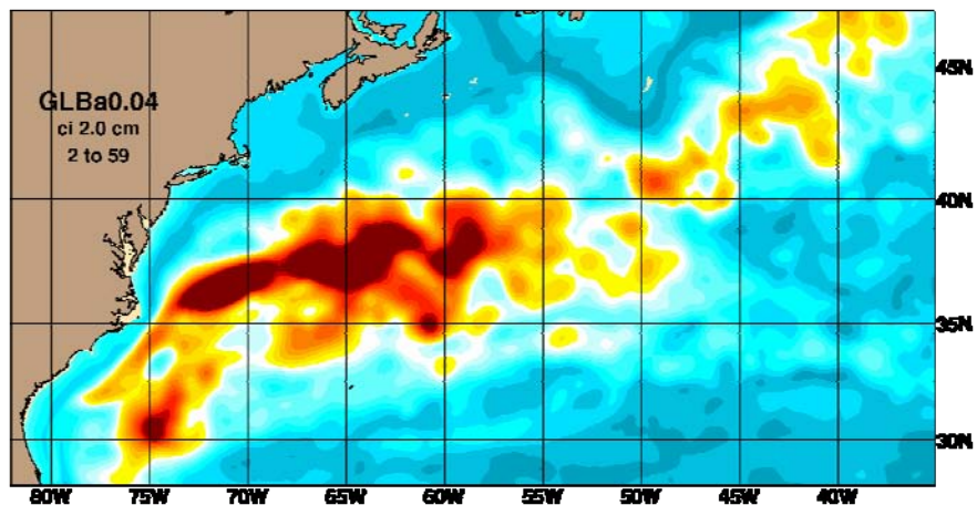
1/25° global HYCOM year 3, Exp. 1.0
