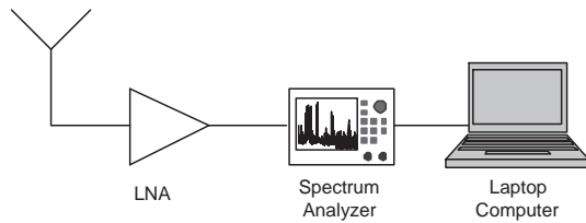
Fig. 1. A block diagram of the Spectrum Occupancy Measurement System.
