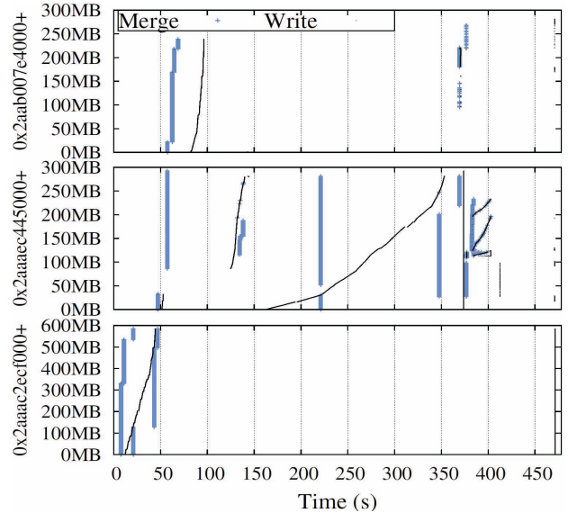
Fig. 25: Representative AMG merge and write profiles
