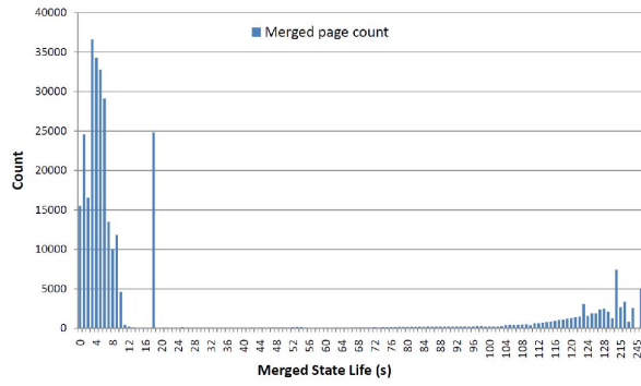
(a) Merged
