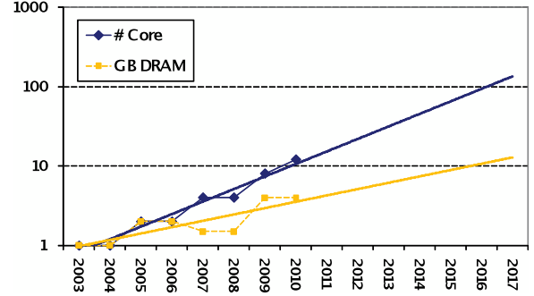
Fig. 1: Memory Capacity Wall
