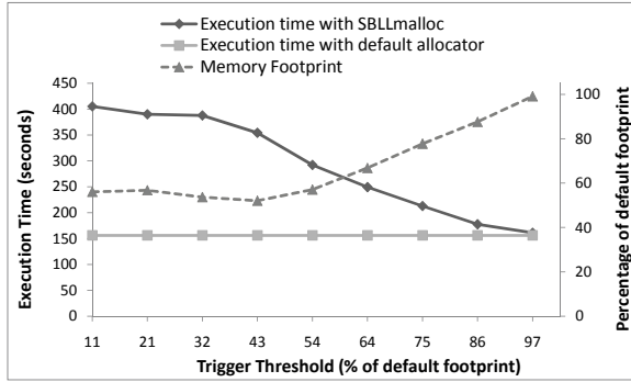
(c) Chombo
