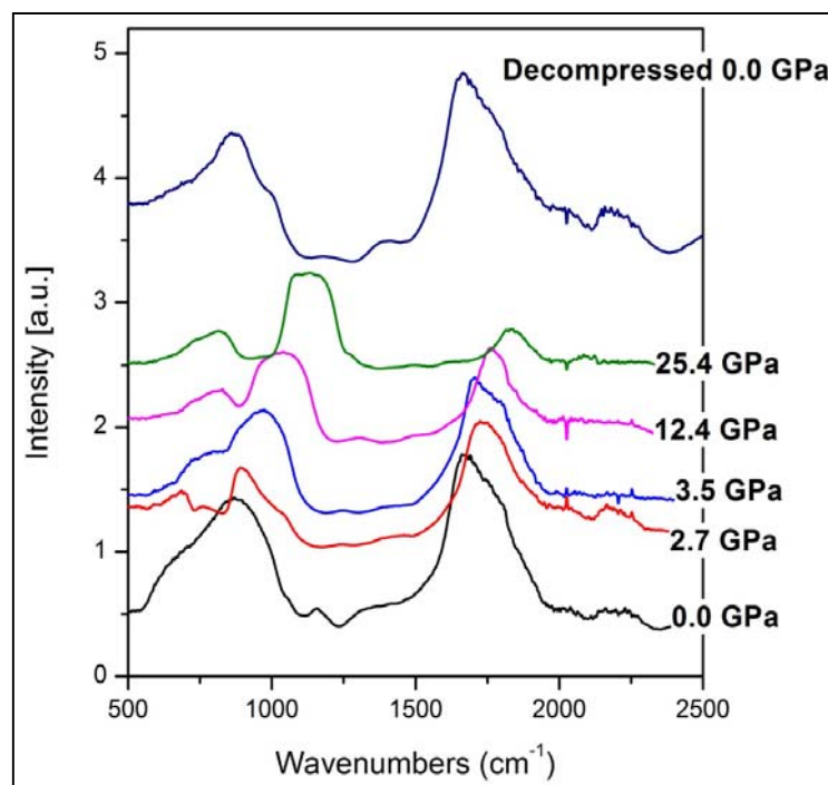
Figure 5. IR spectra of \text{AlH}_3 as a function of pressure in the spectral range between 500 and 2500 \text{cm}^{-1} . Spectra are offset for clarity.
