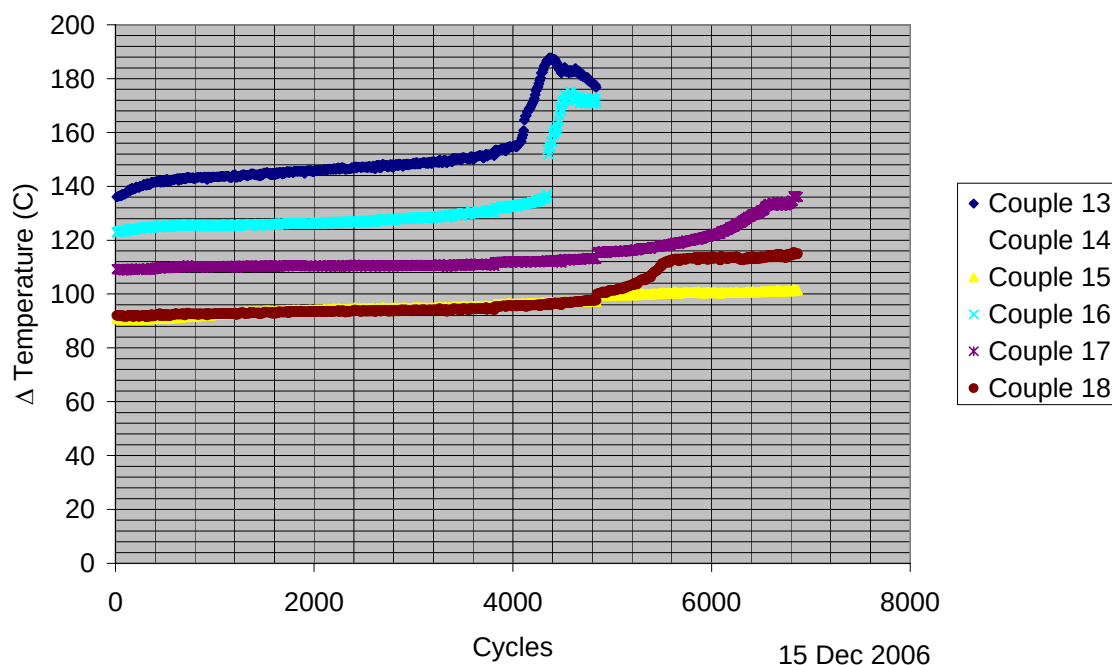
Figure 3. Thermocycling and durability test results of TE materials and shunt assemblies designed for low temperature Bi 2 Te 3 TEG. Heat was applied to the hot side of couples using Joule heating of a resistor, while the cold side was attached to a heat sink maintained at close to ambient temperature. Each cycle lasted 90 seconds. The maximum temperature reached by the hot side during the cycle was recorded. Rising temperature indicates development of a failure.
