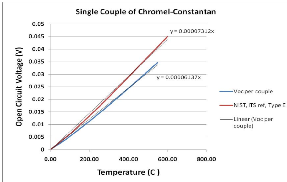
Figure 21. Linear fit to the data shows that output voltage per Chromel-Constantan couple is approximately 61uV/deg C. This value correlates well enough to published values to provide confidence in the behavior of the couples used in this series of testing.
