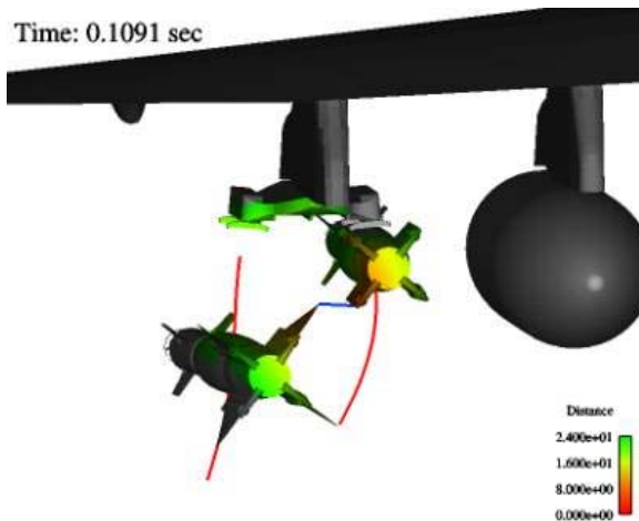
Figure 3 F-18C/GBU-12 Outboard
