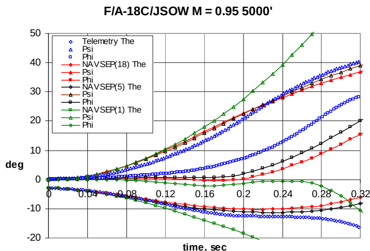
Figure 5 F-18C/JSOW Grid Effects on Trajectory Prediction
