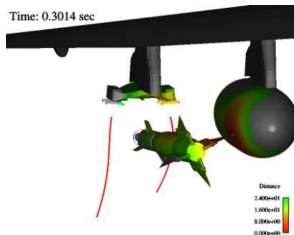
Figure 4 F-18C/GBU-12 Inboard
