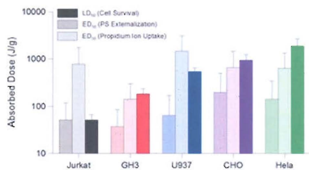
Figure 7. Comparison of ED_{50} for PS externalization and propidium uptake with LD_{50} in different cell lines. Error bars represent the 95% confidence intervals, as calculated from best fit using logarithmic function (see Fig. 2 and 6). doi:10.1371/journal.pone.0015642.g007
