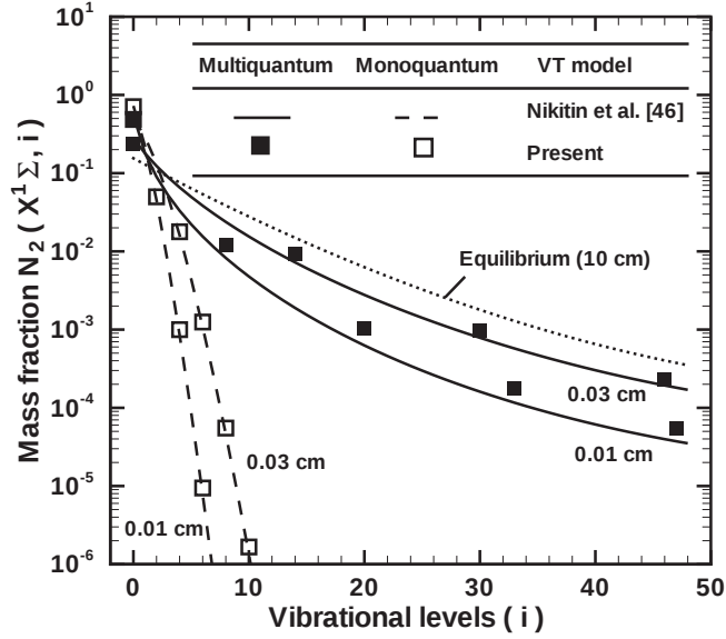
FIG. 7. Vibrational distributions of molecules N_2(X^1\Sigma, i) as functions of the vibrational quantum number i for various distances behind the shock. Multiquantum and monoquantum transitions and various VT models are considered. Free stream conditions: P_\infty = 27 Pa, T_\infty = 300 K, and M_\infty = 19.82 .
