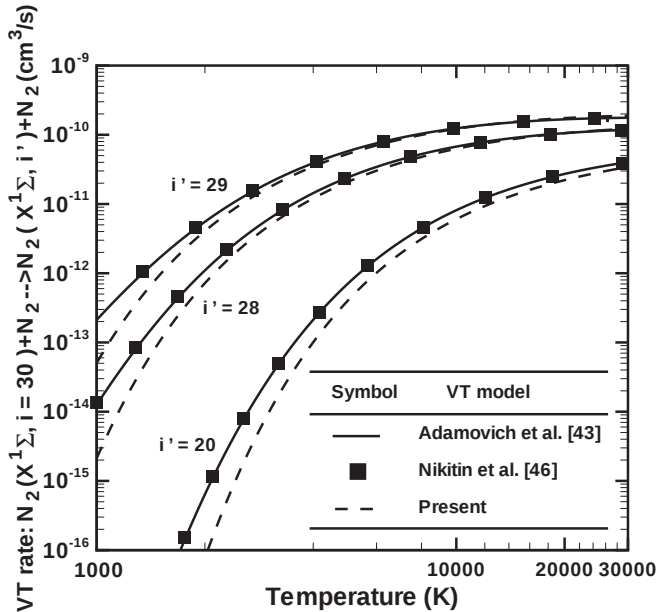
FIG. 4. Multiquantum and monoquantum VT rate coefficients related to N_2(X^1\Sigma, i = 30) + N_2 \rightarrow N_2(X^1\Sigma, i' = 20, 28, 29) + N_2 processes and as functions of the translational temperature. Various VT models are considered.
