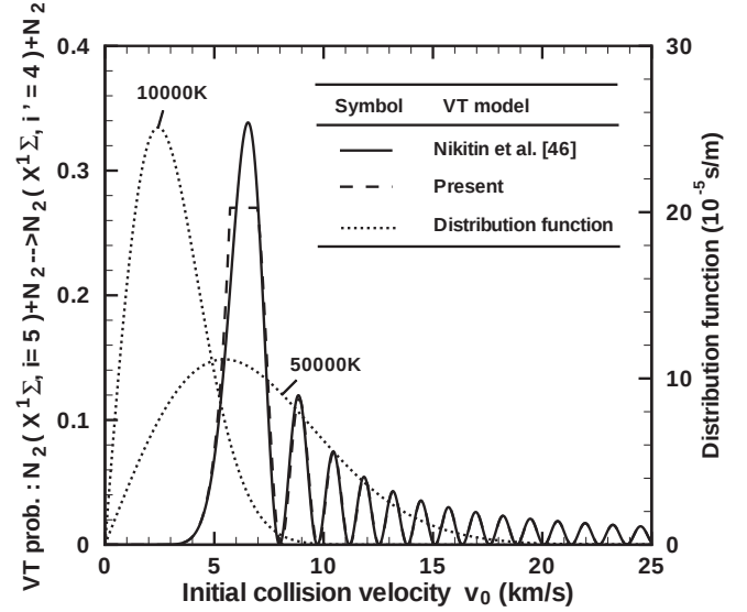
FIG. 1. Monoquantum VT transition probability related to N_2(X^1\Sigma, i=5) + N_2 \rightarrow N_2(X^1\Sigma, i'=4) + N_2 process and the collisional distribution function (for 10 000 and 50 000 K), both as functions of the initial relative velocity v_0 . Various VT models are considered.
