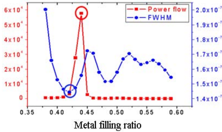
Fig. 1. Filling ratio Vs. normalized power flow and FWHM.
