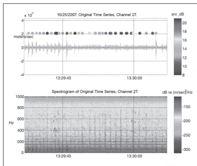
Figure 6. An example of threat activity. The lines in the lower graph (between 10 hertz and 400 hertz) are impacts with a hand tool. The dots above top graph indicate detections made by the TADS algorithm.
