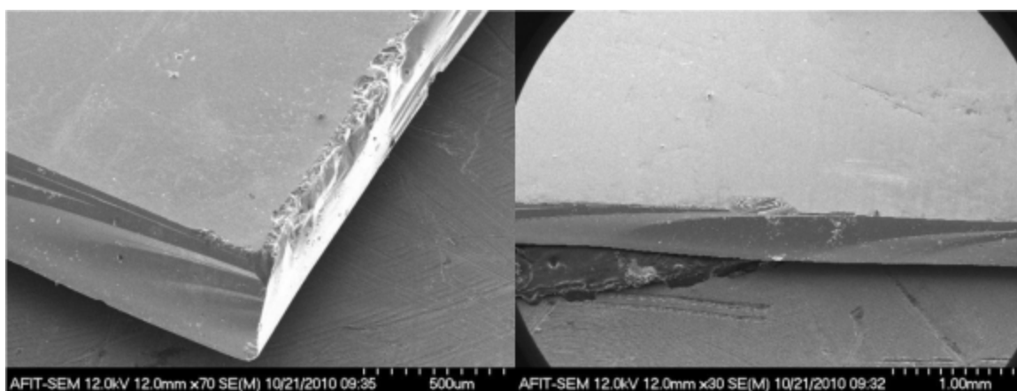
Figure 18. \text{Gd}_2\text{O}_3 on SiC samples. Notice the striations due to the amorphous nature of the substrate. While chipping is visible on the edges, the overall integrity of the sample appears intact.
