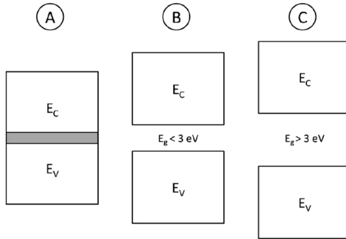
Figure 2. A simplistic depiction of the relationship between the energy bands of different classes of materials. E_C represents the conduction band, while E_V represents the valence band. E_g is the energy gap between the conduction band and the valence band. (A) shows the overlapping energy bands of a typical conductor material. Semiconductors typically have an energy gap of less than 3 eV as shown in (B). Insulator materials have a greater energy gap as shown in (C).
