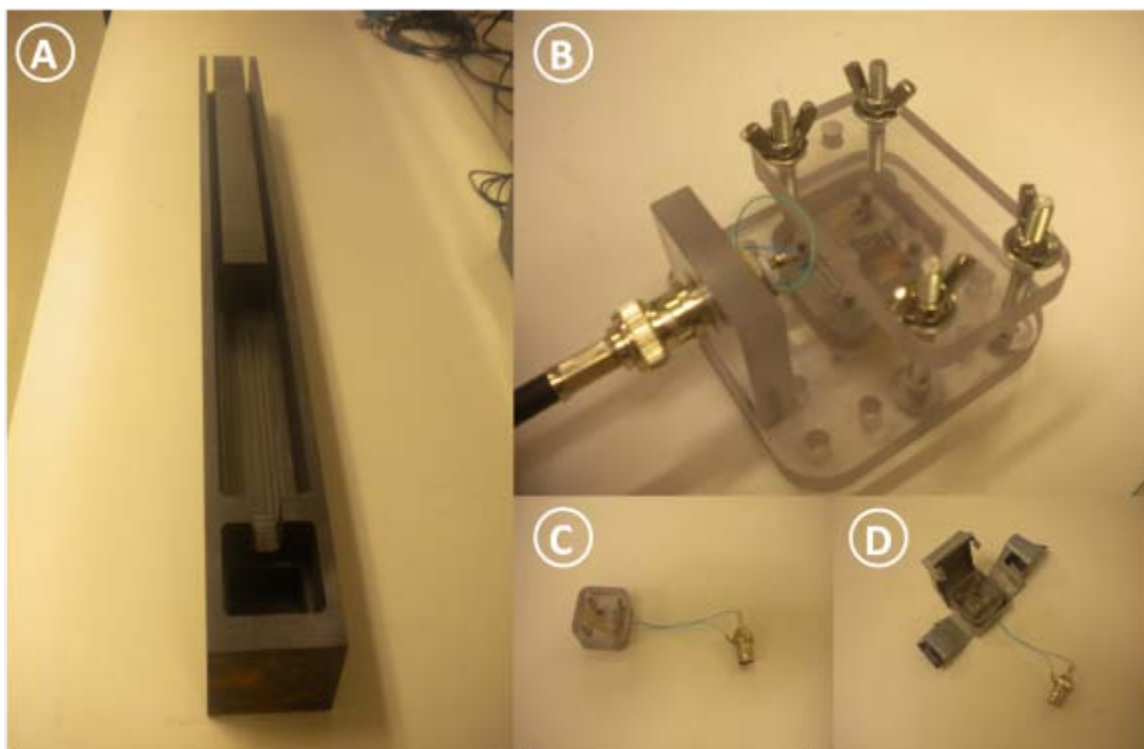
Figure 29. The lower portion of (A) shows the well where the diodes are placed during the experiment. The diodes are packaged in Lexan boxes (C) and then fastened inside a Lexan mount (B) designed to fit in the well shown in (A). (D) shows the diode package in the Cadmium shield. Originally constructed with single wires leading from the conducting posts in the Lexan packages as shown in (B) and (C), the wiring was later changed to RG-174 coaxial cable to eliminate noise induced in the system.
