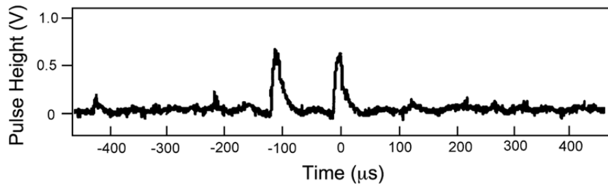
Figure 9. Pulse height train of a Gd doped HfO 2 film on n-type Si substrate diode irradiated with PuBe source neutron flux of approximately 600 \text{ n s}^{-1} \text{ cm}^{-2} . The two large pulses at roughly -100 \mu\text{s} and 0 \mu\text{s} are believed to correspond to the 79 keV IC electron resulting from neutron capture by a Gd-157 nucleus [29].
