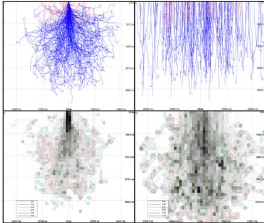
Figure 11. Results from a CASINO simulation of 10^5 79 keV electrons incident on the Gd 2 O 3 on SiC diode. The plots at the top of the figure represent the track of the inbound electrons. The plots below represent energy deposition of the electrons. The plots on the left side of the figure are the results of a simulated beam of electrons, while the right hand plots resulted from a simulated planar flux of electrons.
