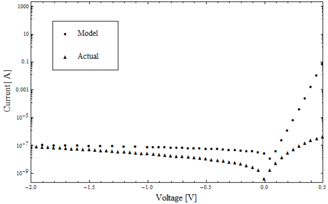
Figure 14. The Davinci model I-V response versus an actual measurement from sample Y3. A generic semiconductor with modified parameters was used to simulate the \text{Gd}_2\text{O}_3 layer.
