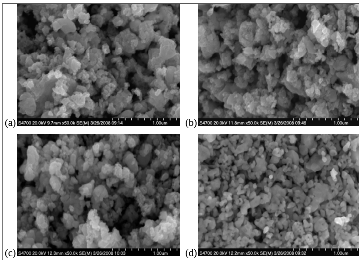
Figure 13. FESEM micrographs of hydrogen reduced compacts (a) unheated, (b) 650, (c) 750, and (d) 850 °C.
