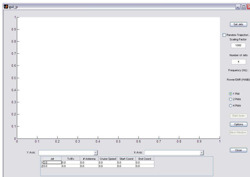
Figure 1: Main Window
