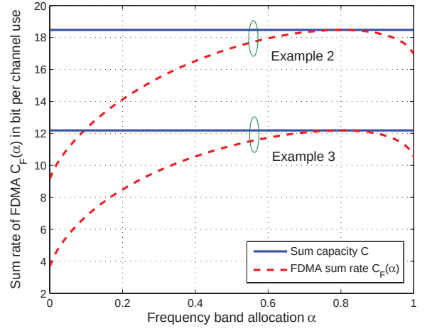
Fig. 1. Sum rate of FDMA versus frequency allocation factor, where, for Example 2 n_r = n_{t1} = n_{t2} = 8 , P_1 = P_2 = 1 , \gamma = 2 , \mathbf{H} and \mathbf{A} are randomly chosen; for Example 3, n_r = n_{t1} = 8 , n_{t2} = 10 , \sigma_1 = \sqrt{3} , \sigma_2 = \sqrt{12} , P_1 = P_2 = 1 , \mathbf{U}_1, \mathbf{U}_2, \mathbf{V}_1 and \mathbf{V}_2 are randomly chosen.
