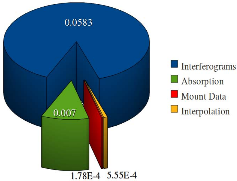
Figure 38. Breakdown of subprocess computational time per frame required to generate one range estimate from one measured interferogram. Numbers displayed in the pie chart have units of seconds per frame. Times were calculated by the algorithm in Appendix C.
