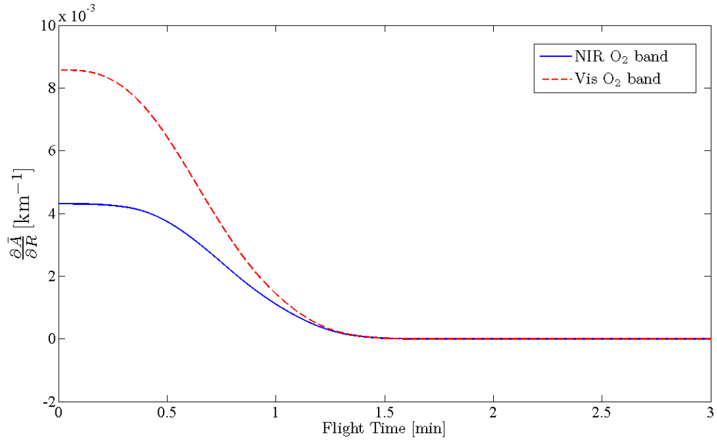
Figure 14. The predicted slope of \bar{A} , with respect to range ( \partial \bar{A} / \partial R ), for a Space Shuttle launch to the International Space Station. Notice that the initial slope of \bar{A} for the Vis O 2 band is twice that of the NIR O 2 band. The slope for both bands quickly falls off towards zero after the first minute of launch.
