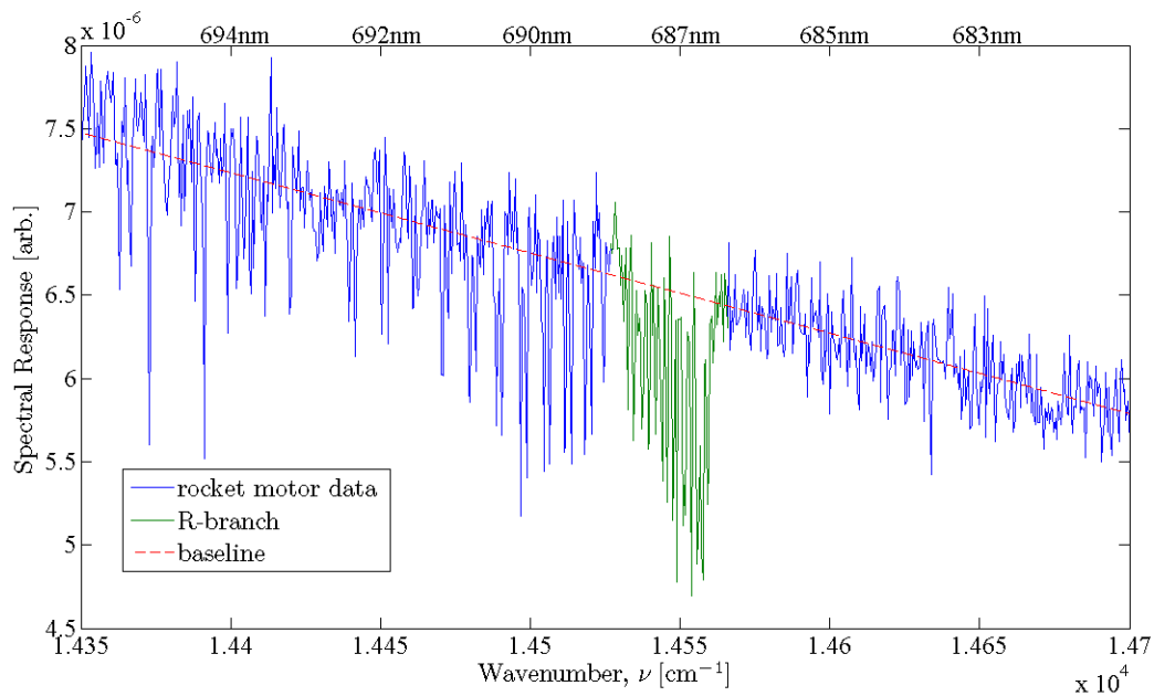
Figure 23. A closeup of the Vis \text{O}_2 absorption band for the static solid rocket motor test. The R-branch is shown in green, while the baseline is shown as the dashed red line.
