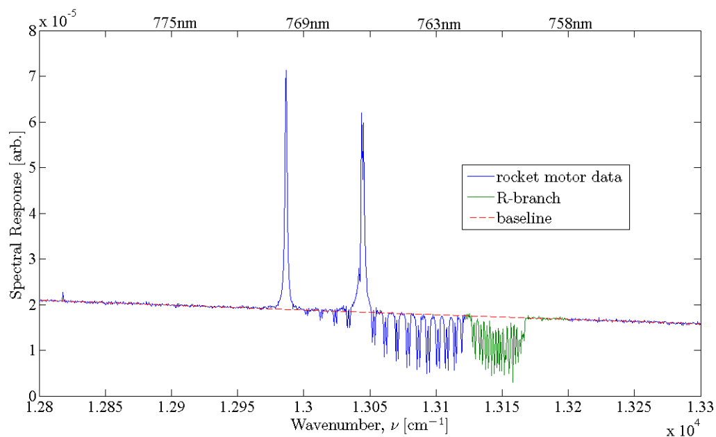
Figure 22. A closeup of the NIR \text{O}_2 absorption band for the static solid rocket motor test. The R-branch is shown in green, while the baseline is shown as the dashed red line. The emission lines are due to alkali metal contaminants in the solid rocket fuel.
