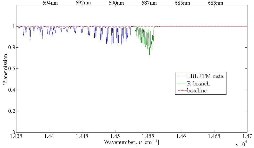
Figure 5. Transmission plot for the Vis O 2 band generated by LBLRTM for a range of 1 km, zenith angle of 89 deg, and altitude of 1 km. The R-branch, used as the in-band data, is shown in green, while the interpolated baseline is displayed as the dashed red line.
