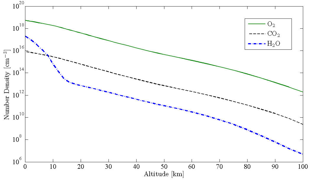
Figure 2. The number density altitude profiles of \text{O}_2 , \text{CO}_2 , and \text{H}_2\text{O} used in the U.S. 1976 Standard Atmosphere. Number density is displayed with a logarithmic axis. Both \text{O}_2 and \text{CO}_2 closely resemble an exponential decaying function, while \text{H}_2\text{O} does not. The tropopause can be seen in the \text{H}_2\text{O} profile near 13 km.
