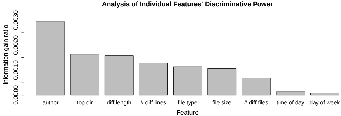
Figure 6.8: The features ordered by decreasing ability to discriminate between security and non-security patches, as represented by the information gain ratio.
