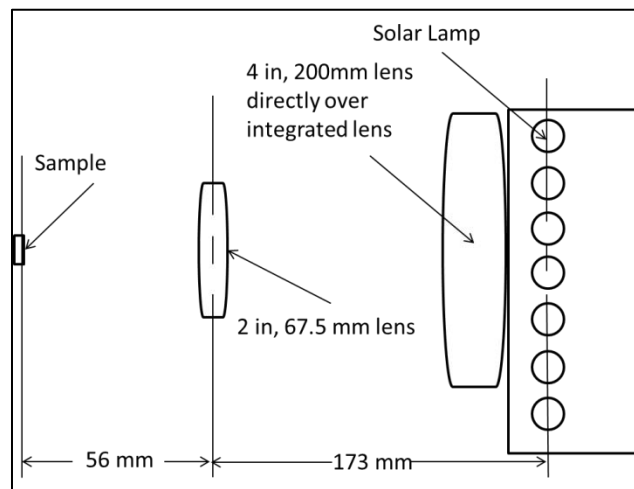
Figure 17. AXTS Setup schematic
