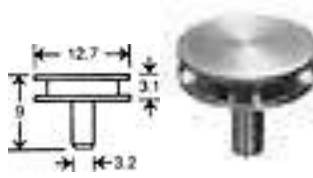
Figure 13. Pella SEM mounting pin, dimensions in mm
