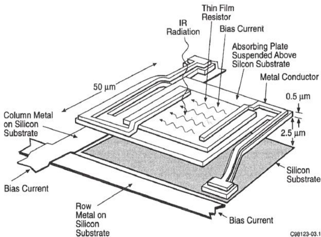
Figure 11. A typical microbolometer cell (Capper et al., 2001)
