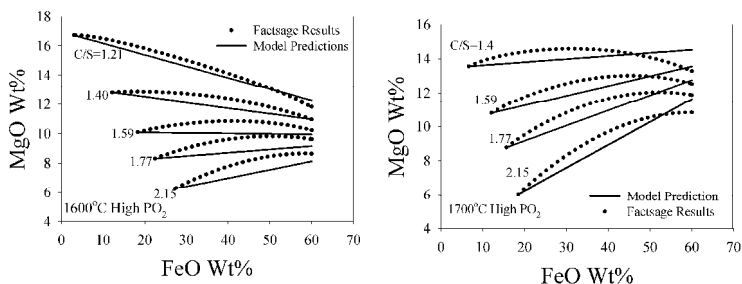
Figure 9 The discrepancy between Factsage calculation results and model assumption for cases at the temperature of a) 1600°C and b) 1700°C in high \text{PO}_2 atmosphere.
