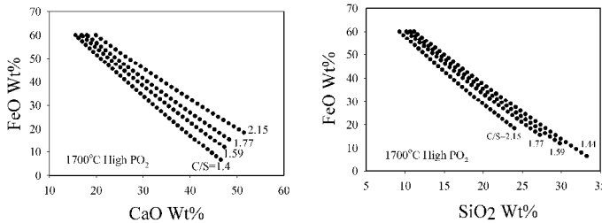
Figure 4 Linear relationship between CaO-FeO and SiO 2 -FeO at different C/S ratios for MgO saturated slag chemistry at 1700°C in high oxygen partial pressure.
