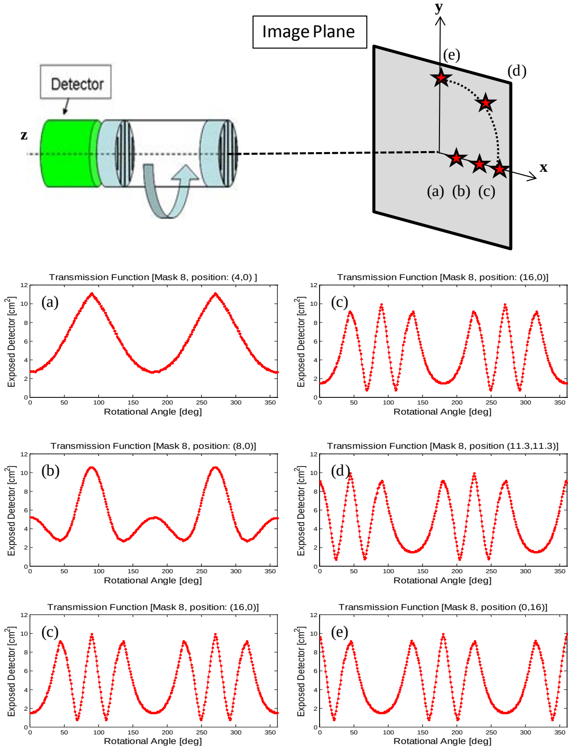
Fig. 3. This shows how the frequency of the transmission function increases as the distance between the source and the RMC centerline increases (a through c) and how the phase of the transmission function shifts based on the degree of rotation from the x axis of the image plane (c through e).
