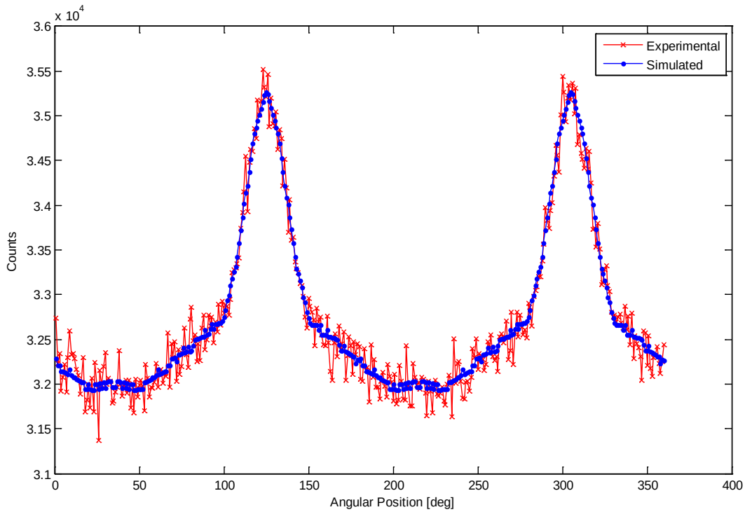
Fig. 26. This plots shows the fidelity comparison between the experimental and simulated transmission function results. Table 2 includes the alterations required to bring the simulated results to align with the experimental. This collection was for mask 3 with a separation distance of 20 cm for 15 hours with the source located at (-10,7).
