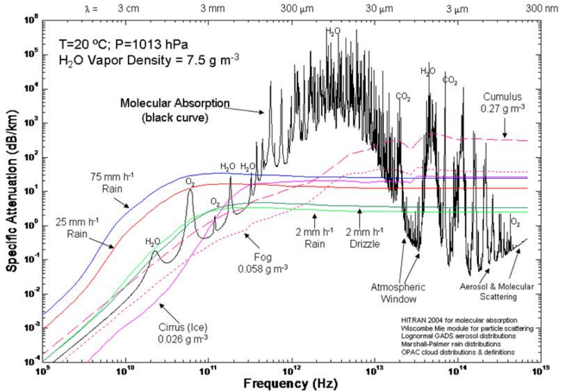
Figure 2. Specific attenuation from 30 cm to \sim 0.4 \mu\text{m} (Adapted Perram, et. al., 2010) The black line is molecular absorption with some effects of continent average aerosols and molecular scattering included. Colored lines represent the specific attenuation that would be added for the hydrometeor distributions shown (rain, clouds, fog). Derived from AFIT LEEDR code.
