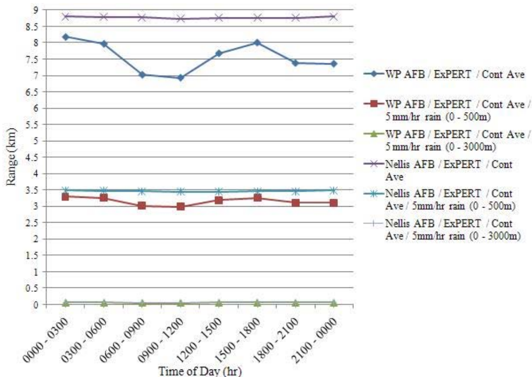
Figure 15. Simulated target lock-on range vs. time of day with and without light rain Plot is based on ExPERT atmosphere, continental average aerosol model, a 50% - average summer, 1.0642 \mu\text{m} laser wavelength, 3,000 meter upper altitude, 5,000 meter laser slant path length, HV 5/7 turbulence model with turbulence multiplier of 1, climatology wind profile.
