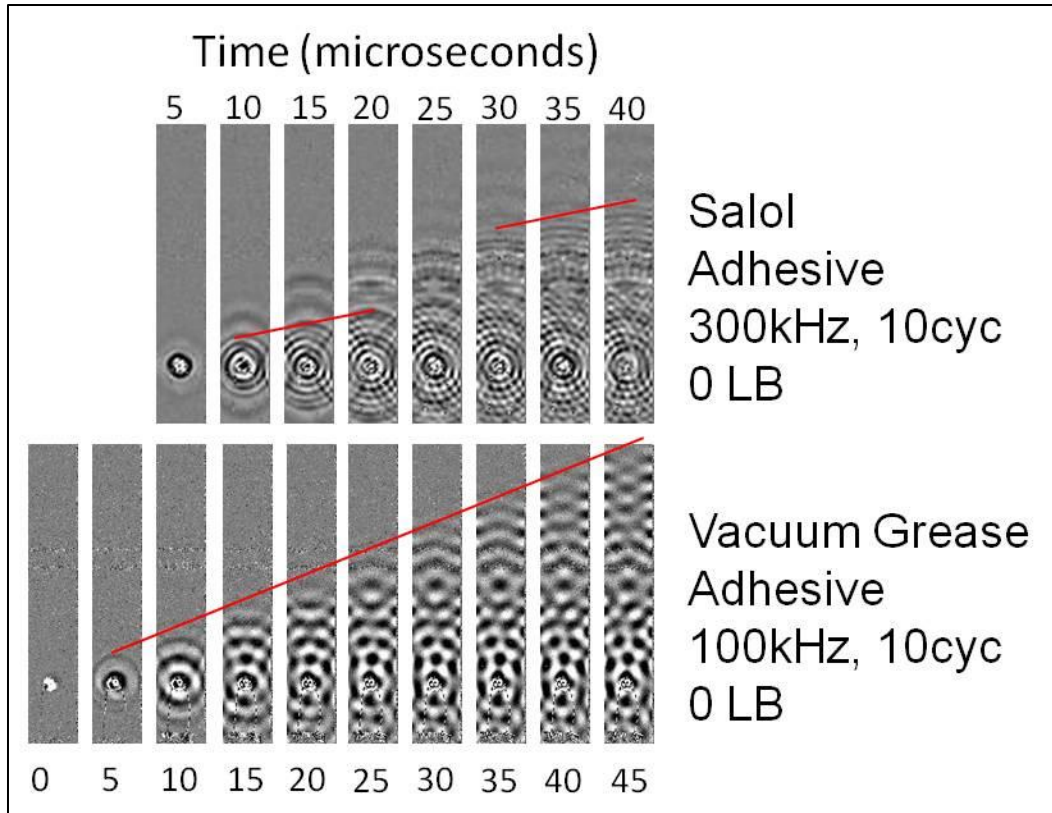
Figure 73 : Laser Vibrometry of Control 1
