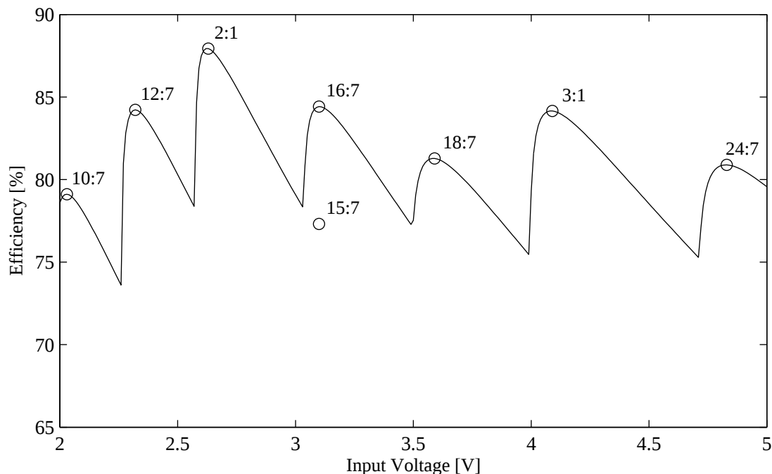
Figure 5.10. Predicted efficiency of multi-ratio converter
