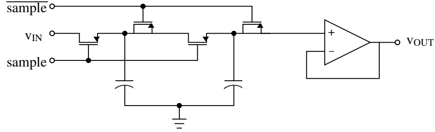
Figure 7.14. Low-leakage sample and hold circuit
