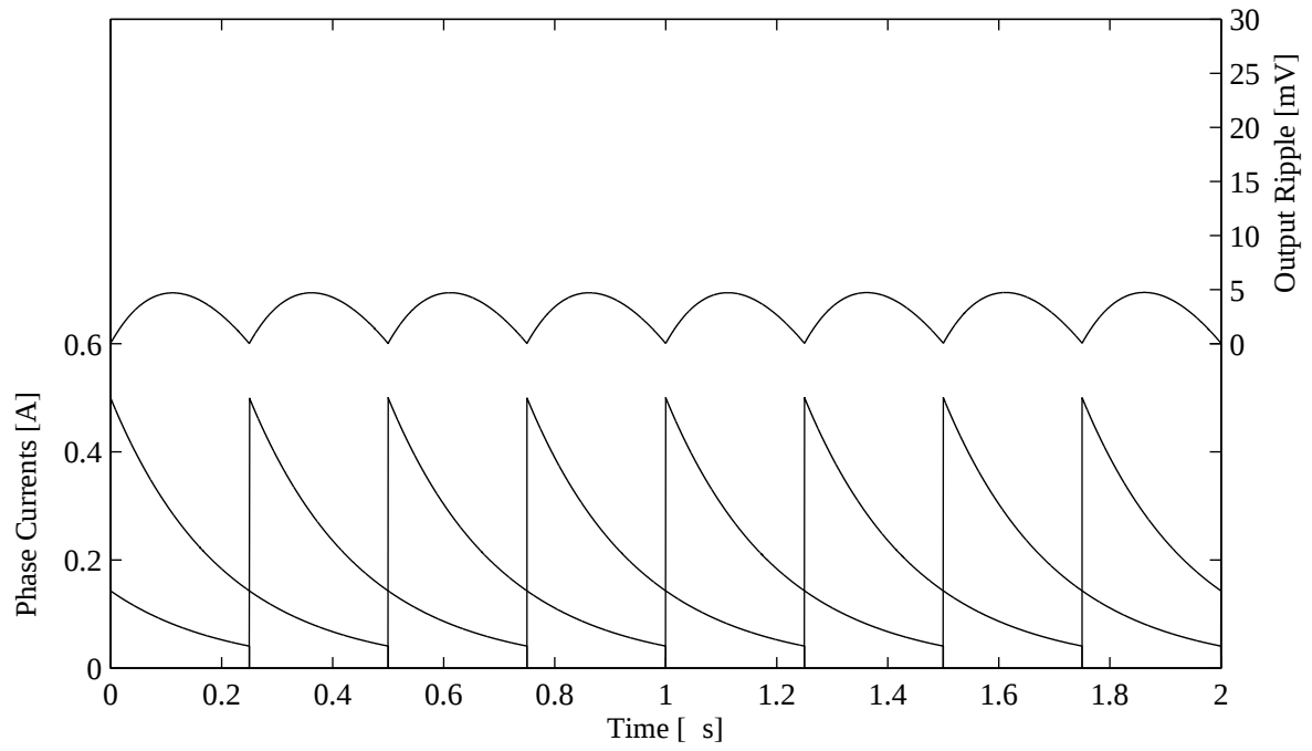
(a) Full load, T = 1 \mu s
