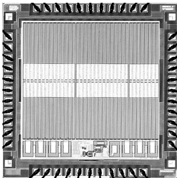
Figure 7.15. Photomicrograph of power interface IC
