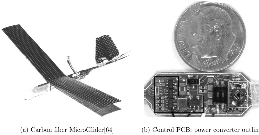
Figure 6.4. Photos of the MicroGlider and control PCB
