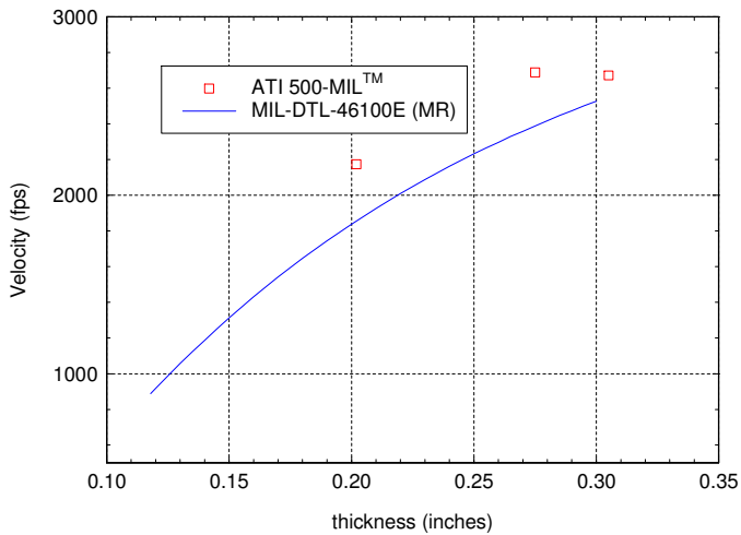
Figure 3. ATI 500-MIL™ Plate Thickness versus V 50 Velocity for the 0.30-Cal APM2 @ 30° Obliquity
