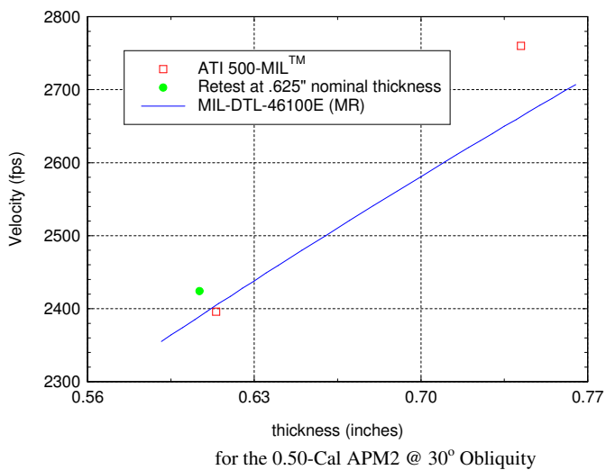
Figure 5. ATI 500-MIL™ Plate Thickness versus V_{50} Velocity for the 14.5mm B32 @ 30° Obliquity
