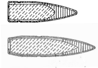
Figure 2. The 14.5-mm BS41 (top) and B32 Test Projectiles (Bottom)
