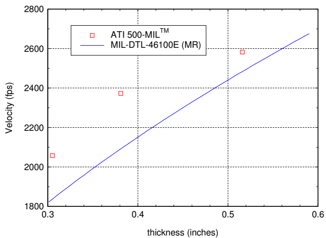
Figure 4. ATI 500-MIL™ Plate Thickness versus V_{50} Velocity
