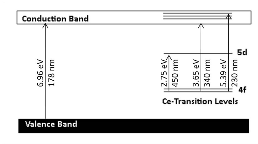
Fig. 11. YAG:Ce energy level diagram adapted from [20].
