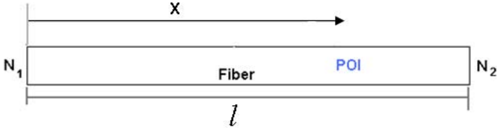
Fig. 10. Double end fiber readout parameters are illustrated. The position of interaction occurs at a distance x from end #1 and a position l - x from end #2. The resulting light yields are N_1 and N_2 , respectively.
