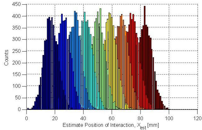
Fig. 73. The simulated position-of-interaction reconstruction data from the 30 cm attenuation is shown as a histogram. The different colors indicate different true positions-of-interaction. The spread in the data (i.e. the standard deviation) is the ideal position resolution.
