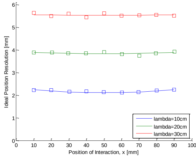
Fig. 86. The achievable position resolution of a 1-MeV (gamma equivalent) scintillation event in a YAG:Ce fiber is significantly improved when readout using a more efficient 100 pixel MPPC as opposed to the inefficient 1600 pixel MPPC used in this research. Any effects of saturation are ignored. Lines indicate the analytical solution and squares indicate the results of Monte Carlo simulations.
