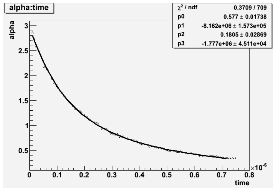
Fiber F6 decay profile data and ROOT two exponential decay fitting parameters.
