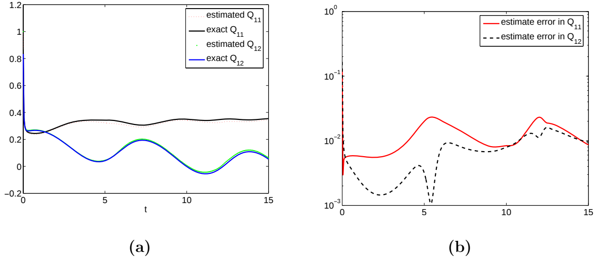
Figure 3: (a) Exact solutions (solid lines) and estimated solutions from UKF (dashed or dotted line) of the Doi model under shear flow with an external force. (b) Corresponding filter errors of UKF in (a).
