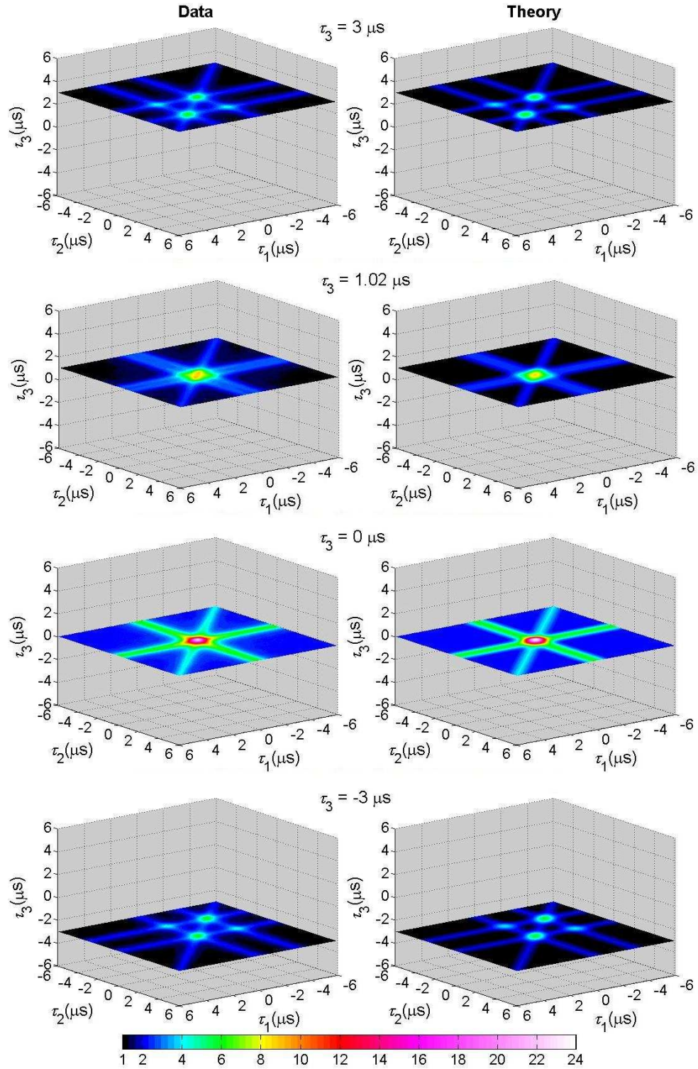
Fig. 4. Four frames from a movie (Media 1) of fourth-order coherence data (left) and theory (right) for the chaotic source for four values of \tau_3 . Color bar at the bottom shows g^{(4)} values.
