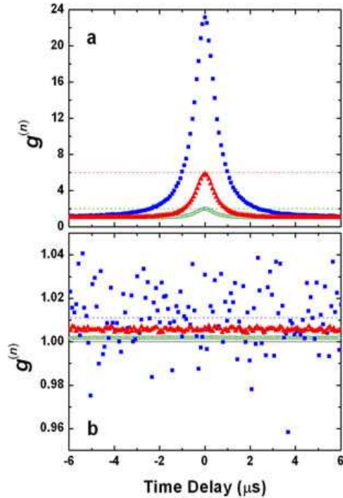
Fig. 2. Measured n^{\text{th}} -order temporal coherences for n = 2 (○), 3 (▲) and 4 (■). (a) Chaotic source data. The magnitude of photon bunching scales roughly as n! , as can be seen from the expected peak g^{(2)} , g^{(3)} and g^{(4)} values of 2 (dashed green line), 6 (dashed red line) and 24 (top axis). (b) Laser source data, also showing the expected value of 1 (black line) and the mean measured g^{(4)} value of 1.011 (dashed blue line). In both (a) and (b), the g^{(2)} data are displayed as a function of \tau , while the g^{(3)} and g^{(4)} data are plotted against parameterized delays that measure temporal distance from the origin, \tau_{P3} = \pm (\tau_1^2 + \tau_2^2)^{1/2} and \tau_{P4} = \pm (\tau_1^2 + \tau_2^2 + \tau_3^2)^{1/2} , respectively, where \pm is determined by the sign of \tau_1 . These trace out cross sections from (\tau_1, \tau_2) = (-6/\sqrt{2} \mu\text{s}, 6/\sqrt{2} \mu\text{s}) to (6/\sqrt{2} \mu\text{s}, -6/\sqrt{2} \mu\text{s}) and (\tau_1, \tau_2, \tau_3) from (-4 \mu\text{s}, 2 \mu\text{s}, 4 \mu\text{s}) to (4 \mu\text{s}, -2 \mu\text{s}, -4 \mu\text{s}) .
