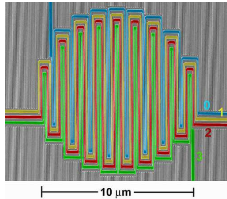
Fig. 1. Scanning-electron microscope image of the four-element SNSPD, with nanowire elements 0-3 traced out in color. Each element consists of a ~5 nm-thick \times 80 nm-wide NbN nanowire on a sapphire substrate, with 60 nm gaps between wires. The 9.4 \mu m-diameter active area is well matched to the spatial mode of a single mode optical fiber, the cleaved end of which is held within ~10 \mu m of the detector surface. The interleaved design ensures that all four elements equally sample this spatial mode.
