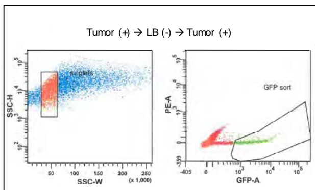
Figure 2. Identification of fluorescent bacteria by FACS
