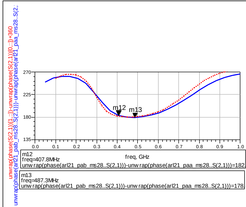
Figure 10. ADS S-parameter simulation (dotted) of ARL21M425 BPSK phase A/B versus measurement (solid).
