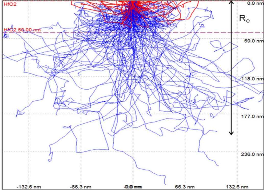
Figure 8. Sample Monte Carlo simulation using an electron beam energy of 5 keV and a sample of HfO 2 that is 50 nm thick with a density of 9.68 g/cm 3 . The arrow indicates the calculated penetration depth, R_e , given by equation (2.15) and also illustrated in Figure 6.
