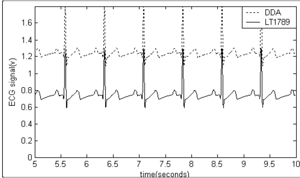
Figure 10. The amplified simulated ECG from our DAA and LT1789 (Linear Technology, Inc).
