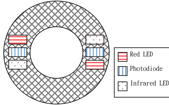
Figure 1. An O-shaped NIR sensor integrating LEDs and PDs.
