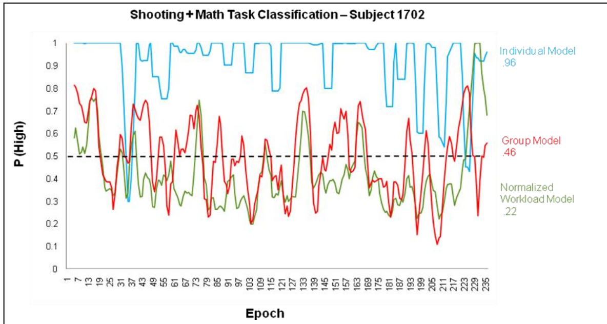
Figure 15. Classifier output over the course of the S&M task for a single subject.
