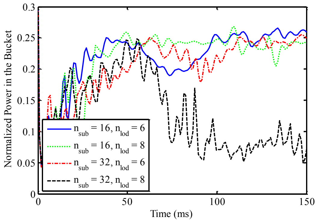
Figure 68. Spatial resolution study to determine insipient PCI for ab initio phase compensation with time-dependent thermal blooming and a distortion number, N_D=33.6 rad, using a.) peak Strehl ratio versus time and b.) normalized power in the bucket versus time.
