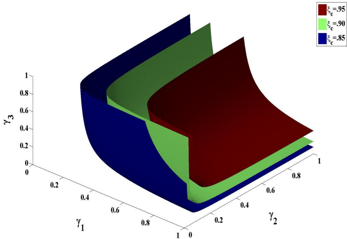
Figure 5.11: Enzyme Combinations for Different Critical Thresholds Based on I_0=100 nM, t_e = 2 sec, T = 350^\circ\text{C} , \alpha=10 , \beta=3 , t_0 = 250 sec, and values from Table 5.1 and 5.2.
