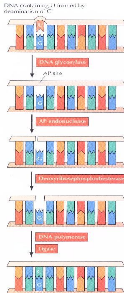
Figure 5.1: Base Excision Repair [3]
