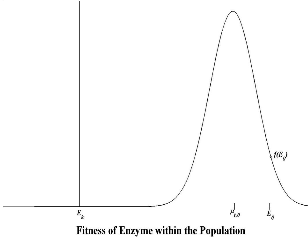
Figure 4.1: Enzyme Fitness Prior to Any Heating
