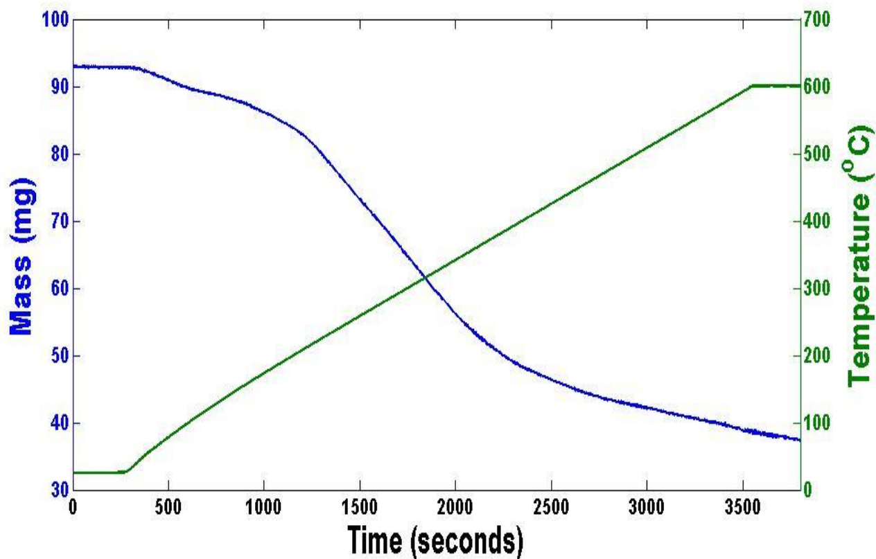
Figure 3.1: TGA Raw Data
