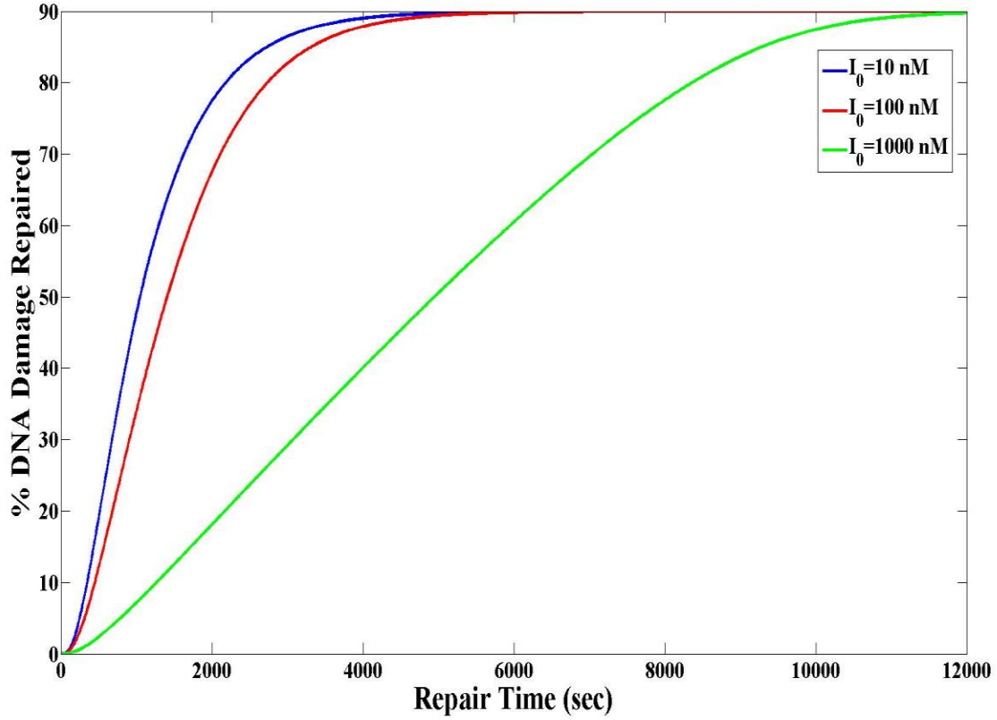
Figure 5.5: DNA Repair Analysis when 90% of DNA & Enzymes are Damaged
