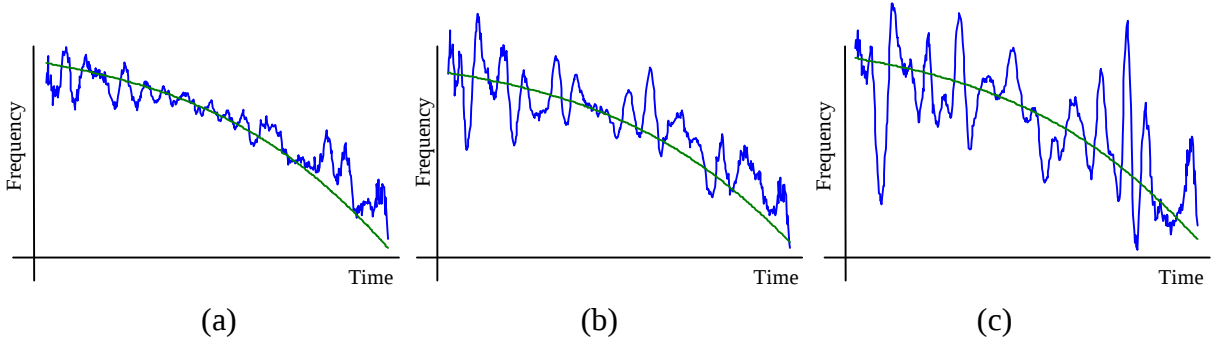
Fig. 16 Estimation of Doppler shift using features from wavelet-generated video and pattern recognition neural networks (nonlinear change in shift over time): (a) signal-to-noise ratio of -0.5 dB, (b) signal-to-noise ratio of -2 dB, (c) signal-to-noise ratio of -4 dB.
