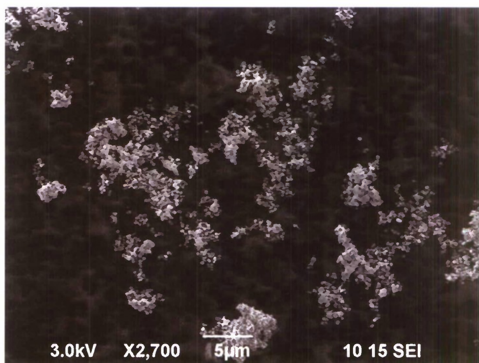
Figure 10 - SEM Image #2 of Diphenyldimethoxysilane Coated TiO 2
