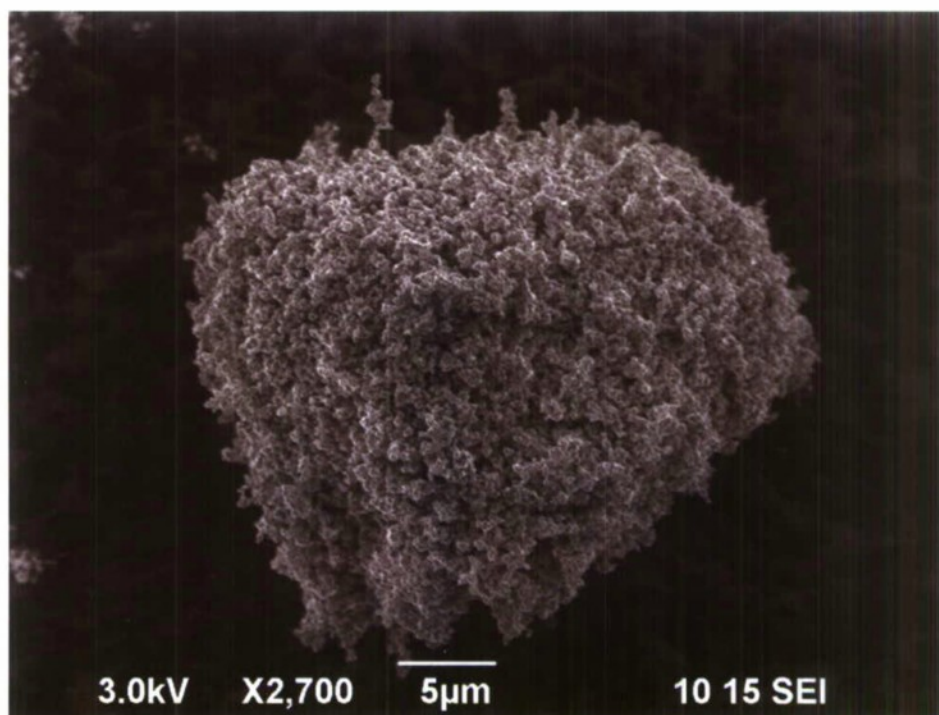
Figure 9 - SEM Image #1 of Diphenyldimethoxysilane Coated TiO 2
