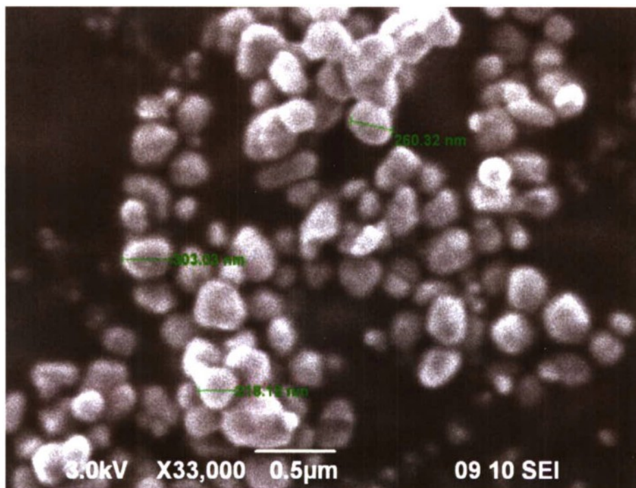
Figure 11 - SEM Image #3 of Diphenyldimethoxysilane Coated \text{TiO}_2
