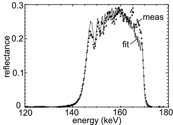
Figure 9.19: Reflectance of a depth-graded W/SiC multilayer measured at 2.09 mrad grazing angle (Windt et al 2003).
