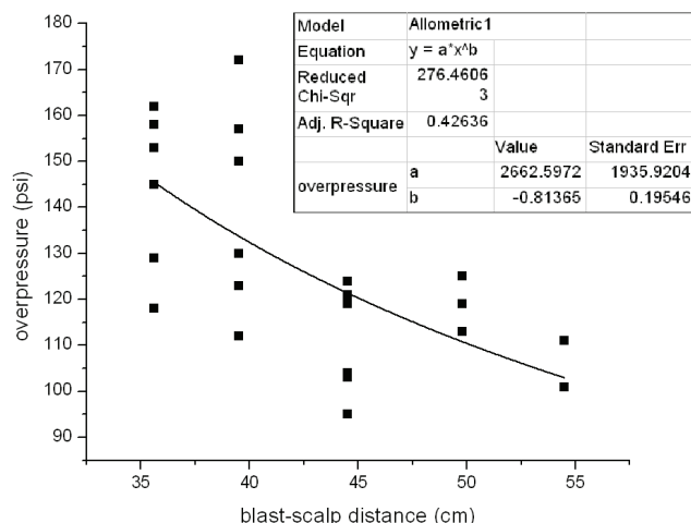
Fig. 4. Peak blast overpressures generated by COBIA with various sizes of BDC. Values shown are for power level 2 shots only, with values plotted against the blast-to-scalp distance. A least-squares fit of the data to a power function is also shown (solid line).
