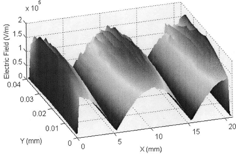
Figure 4-7: Magnitude of the electric field versus XY position at second resonance.
