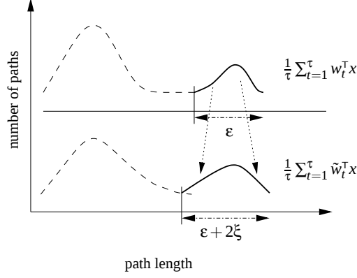
Figure 4: Illustration of the second inclusion in Lemma 4.2. The set of \epsilon -longest paths, the object of interest, is contained in the set of (\epsilon + 2\xi) -longest paths w.r.t. to the sequence \tilde{w}_1, \dots, \tilde{w}_\tau . Under a margin assumption, equality between the two sets can be shown, as exhibited by Theorem 4.2.
