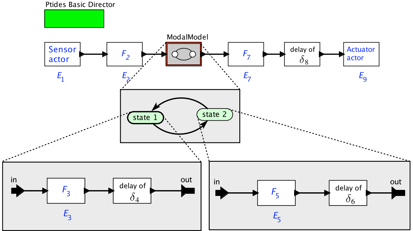
Figure 5. Specifying model delay
