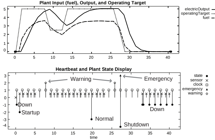
Figure 7. Power plant output and events
