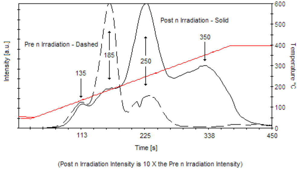
Figure 39. TL bulk glow curve comparison of \text{Li}_2\text{B}_4\text{O}_7\text{:}^6\text{Li} pre- and post-n irradiation, with thermal n interaction density of 10^{15} \text{ cm}^{-3} .
