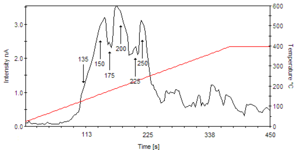
Figure 21. TL glow curve for \text{Li}_2\text{B}_4\text{O}_7: {}^6\text{Li} above room temperature post fast neutron irradiation to a interaction density of 10^{15} \text{ cm}^{-3} .
