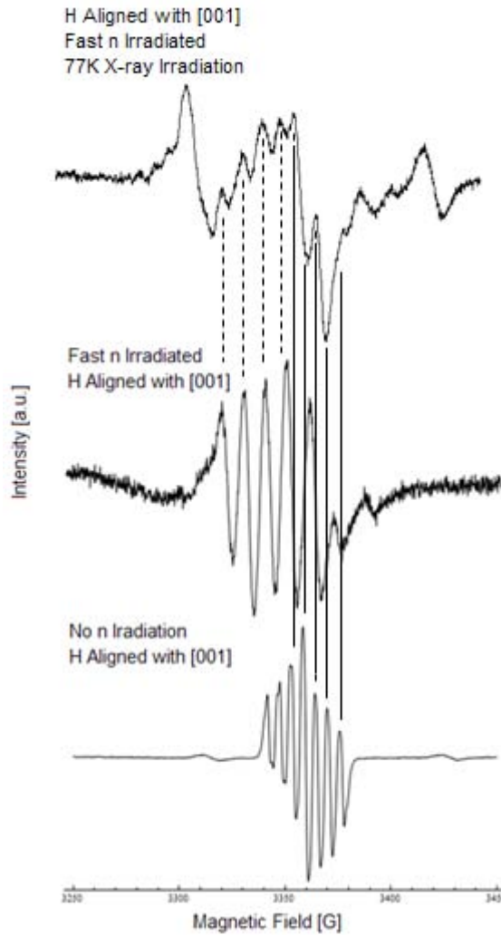
Figure 38. EPR spectra comparison pre and post neutron irradiation for \text{Li}_2\text{B}_4\text{O}_7: ^6\text{Li} crystal. EPR spectra for neutron irradiated crystal obtained at 12 K. EPR spectra for pre-neutron irradiated crystal obtained at 77 K. Top spectrum and bottom spectrum were both x-ray irradiated at 77 K. Dashed and solid lines show the position of the combined lines in the top spectrum.
