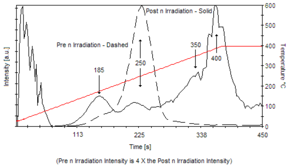
Figure 40. TL bulk glow curve comparison of \text{Li}_2\text{B}_4\text{O}_7\text{:}^{10}\text{B} pre and post n irradiation, thermal n interaction density of 10^{17} \text{ cm}^{-3} .
