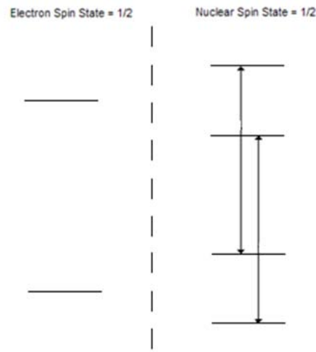
Figure 4. The available energy levels and strongly allowed transitions, \Delta M = \pm 1 , \Delta m = \pm 0 , of an unpaired electron on a spin \frac{1}{2} nucleus.
