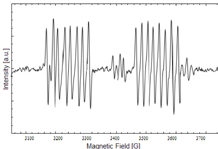
Figure 31. EPR spectrum of \text{Li}_2\text{B}_4\text{O}_7:\text{Ag} the magnetic field is aligned with the [001]. The spectrum was taken at 30 K. The crystal was x-ray irradiated at room temperature to populate charge traps. Spectrum is an enhancement of the region between 3050 – 3750 G.
