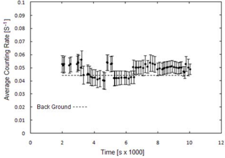
Figure 35. Average 511 keV gamma radiation count rate for \text{Li}_2\text{B}_4\text{O}_7\text{:}^{10}\text{B} after n irradiation in the AFIT pile to secular equilibrium. The dashed line is the average count rate pre-neutron irradiation for 511 keV gamma radiations.
