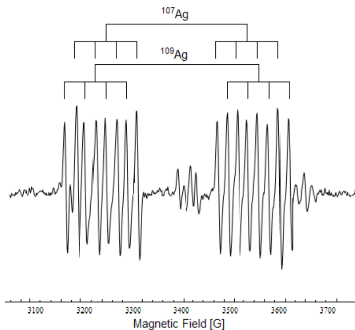
Figure 41. EPR spectrum of \text{Li}_2\text{B}_4\text{O}_7:\text{Ag} the magnetic field is aligned with the [001]. The spectrum was taken at 30 K. The crystal was x-ray irradiated at room temperature to populate charge traps. The stick diagram shows the resolved isotopes of Ag.
