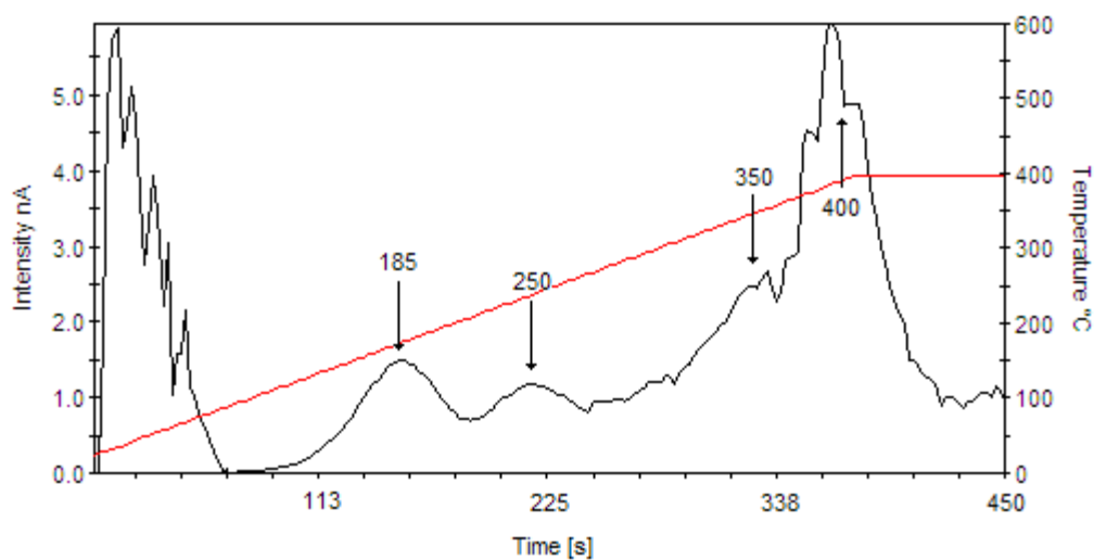
Figure 22. TL glow curve for \text{Li}_2\text{B}_4\text{O}_7: {}^{10}\text{B} above room temperature post thermal neutron irradiation to a interaction density of 10^{17} \text{ cm}^{-3} .
