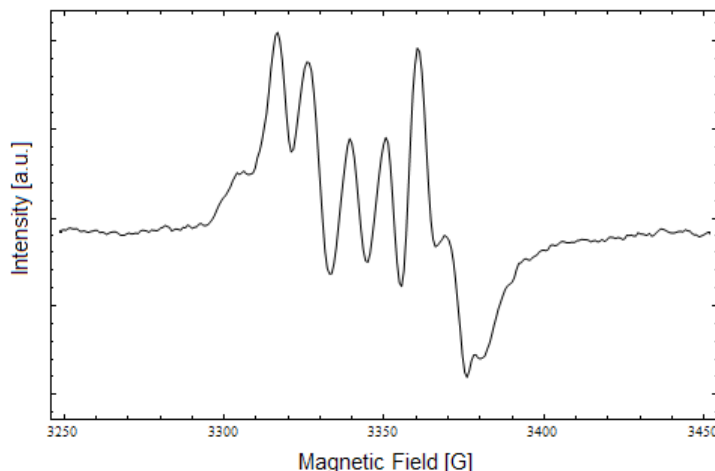
Figure 18. EPR spectra of \text{Li}_2\text{B}_4\text{O}_7\text{:}^6\text{Li} thermal neutron irradiated to an interaction density of 10^{17} \text{ cm}^{-3} . The magnetic field is aligned near the [001], the spectra were taken at 12 K.
