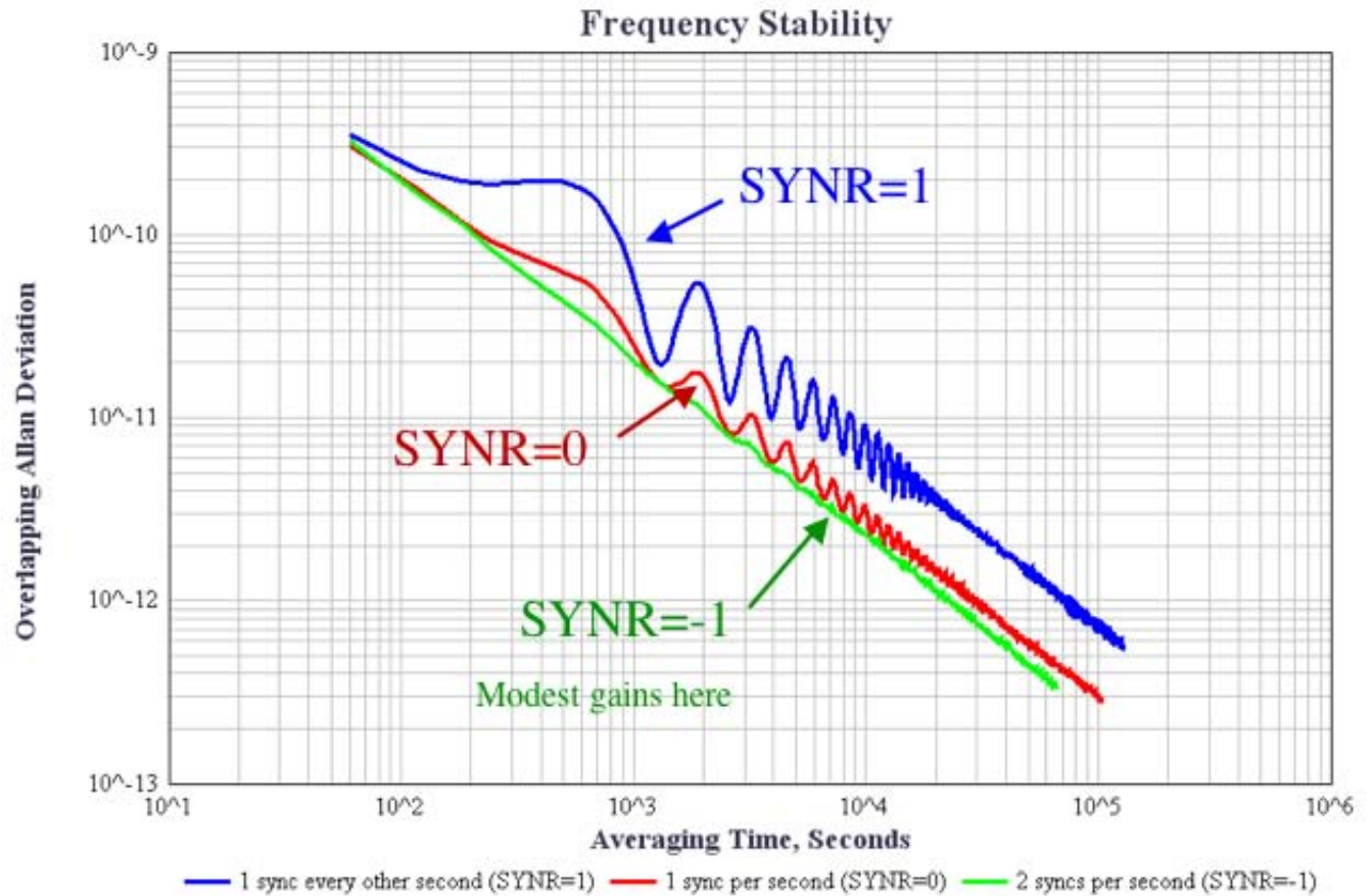
Figure 11. Overlapping Allan deviations, effect of varying PTP synchronization messaging interval.
