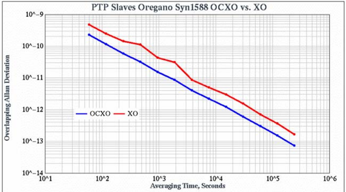
Figure 6. Overlapping Allan deviation, Oregano Syn1588PCIE OCXO vs. XO.
