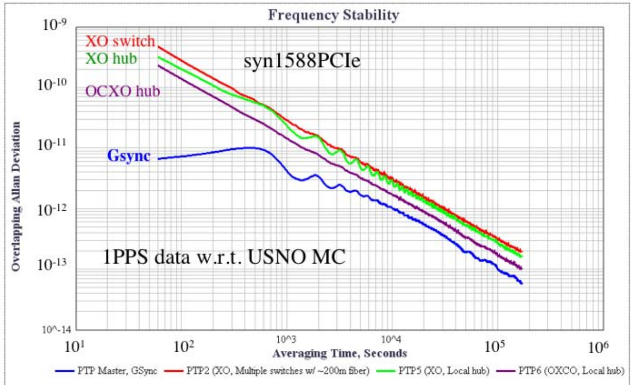
Figure 9. Overlapping Allan deviations, comparing operation through a switch vs. a hub, and with OCXO.
