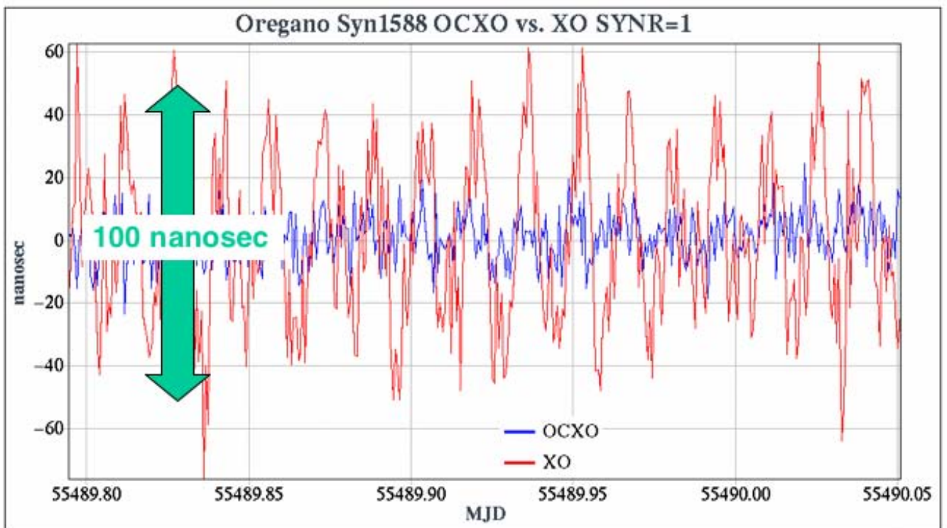
Figure 5. Comparison of phase error of the standard Syn1588PCIe (red) with the OCXO version (blue).
