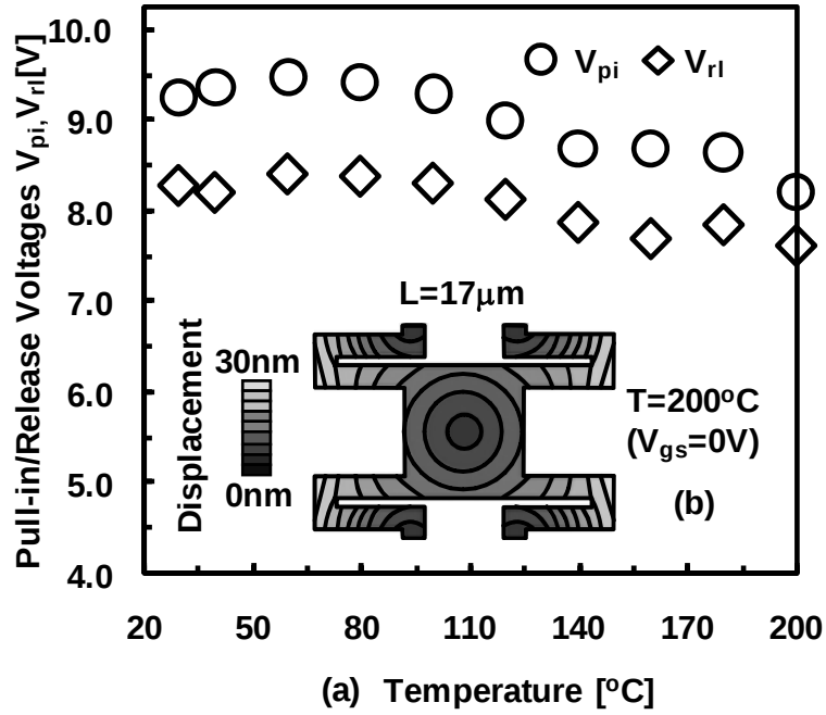
Fig. 4.12 a) Measured V_{pi} and V_{rl} vs. T for L=17\mu m . (b) ANSYS shows that the folded spring design releases the thermal/residual stress by expansion.
