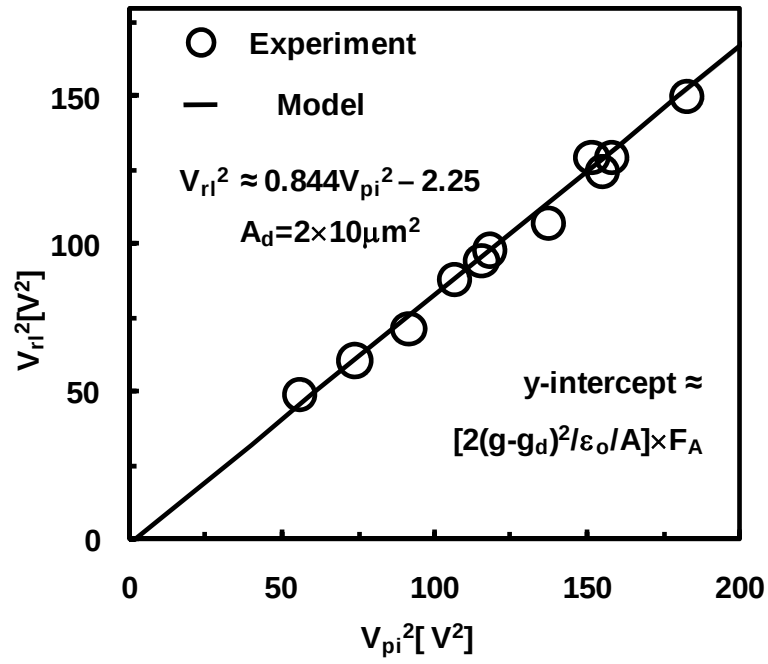
Fig. 4.10 V_{r1}^2 vs. V_{pi}^2 for the relays of Fig. 4.9. F_A is extracted to be 0.45 \mu N .
