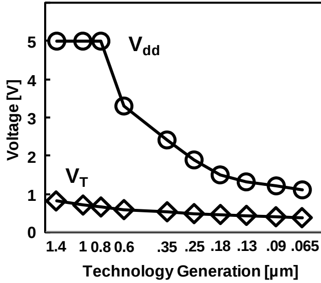
Fig. 1.2 To maintain constant power density, both the supply and the threshold voltages of a CMOS integrated circuit should be reduced along with the lithographic dimension of CMOS transistors. But due to MOSFET subthreshold leakage, both V_{dd} and V_T scaling have slowed down in recent technology generations [1.1].
