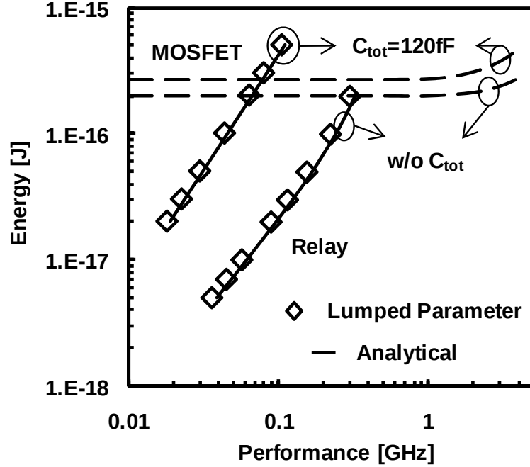
Fig. 5.8 Simulated energy-performance comparison of the MOSFET vs. relay, for a 30-stage FO4 inverter chain / relay chain (average transition probability =0.01) [8]. MOSFET parameters are taken from the ITRS, for the 65nm LSTP technology node. Relay parameters are tabulated in Table II. The minimum energy is set by \Gamma . Notice that due to the low air-gap capacitance, relay performance is more sensitive to load capacitance than the MOSFET [8].
