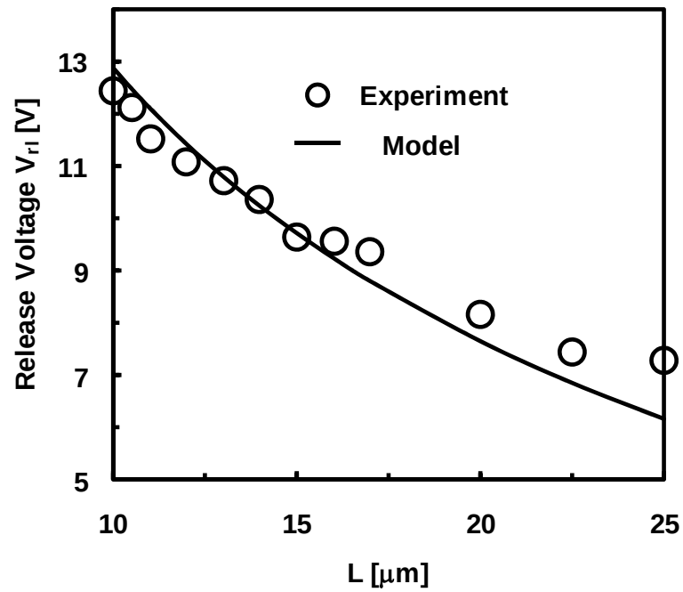
Fig. 4.11 Measured relay V_{r1} vs. L . The measured data is within 10% of the analytical model.
