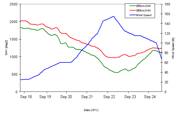
Fig. 4. Hurricane Rita (2005): time series of the best track intensity (kt) from the National Hurricane Center best track data (blue), DAV time series using a radius of 250km (green) and 350km (red). During the course of the time series 0000 local is between 0500 UTC and 0600 UTC.
