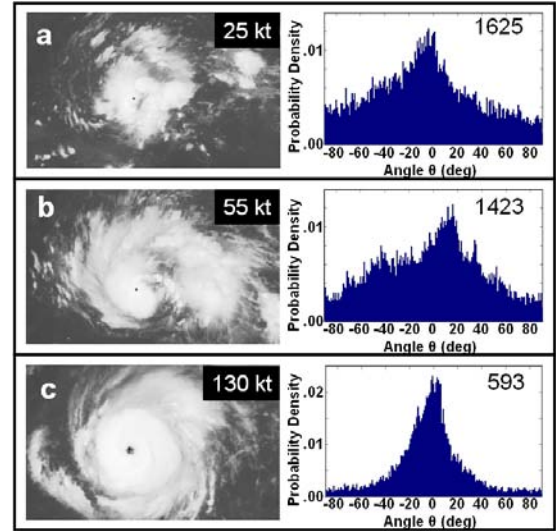
Fig. 2: Sequence of infrared images and deviation angles histograms for Hurricane Rita (2005): a) 0815 UTC 18 September 2005. Intensity: 25kt, 1009 hPa, DAV: 1625 \text{deg}^2 ; b) 1415 UTC 19 September 2005. Intensity: 55 kt, 997 hPa, DAV: 1423 \text{deg}^2 ; and c) 1415 UTC 21 September 2005. Intensity: 130kt, 932 hPa, DAV: 593 \text{deg}^2 .
