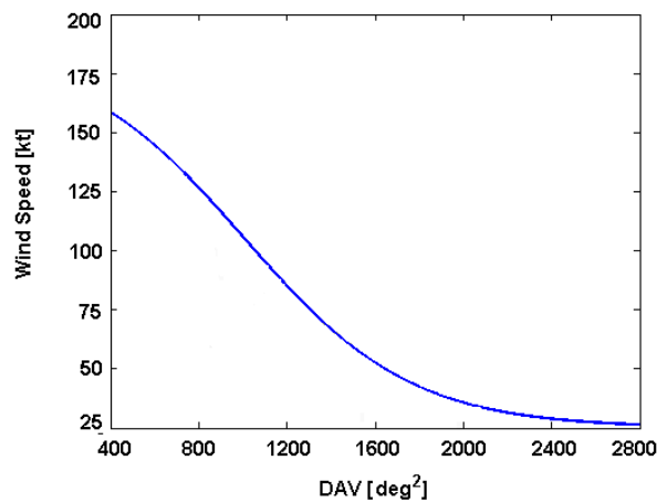
Fig. 5: 350km DAV vs best-track intensity estimates over 2004-2008 for the Atlantic basin.
