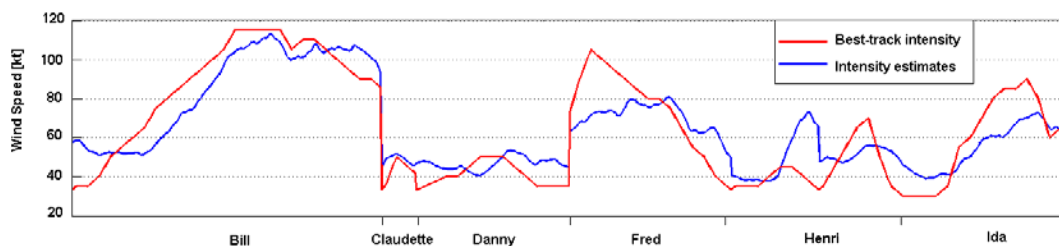
Fig. 6. Estimate intensity results for 2009 using 2004 to 2008 to training the system. The RMSE is 12.9 kt.
