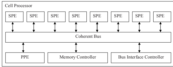
Figure 1. IBM Cell BE processor architecture.
