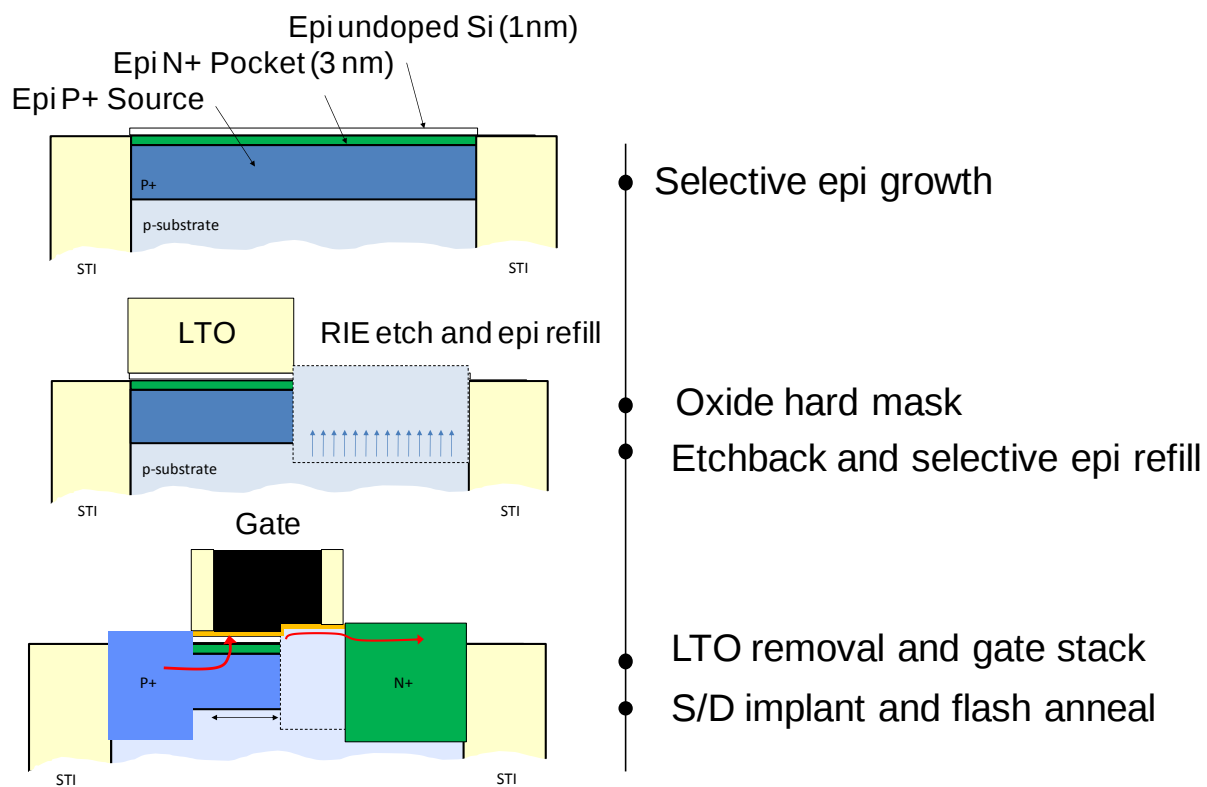
Figure 6.1: Proposed process flow for future gTFET experiment utilizing epitaxial growth. This design addresses dielectric interface quality concerns with an undoped capping layer. The lateral doping profile is made as abrupt as possible from reactive ion etching.
