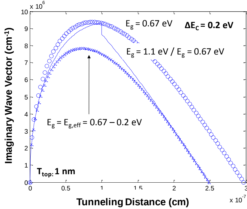
Figure 2.10: Imaginary wave vector along tunneling path for three structures. (1) Semiconductor of E_g = 0.67 eV (2) Hetero-structure of 1nm E_g = 1.1 eV atop E_g = 0.67 eV with conduction band offset of 0.2 eV. (3) Semiconductor of E_g = E_{g,eff} = 0.67 - 0.2 = 0.47 eV. Tunneling across the hetero-structure is similar to tunneling in an E_{g,eff} material.
