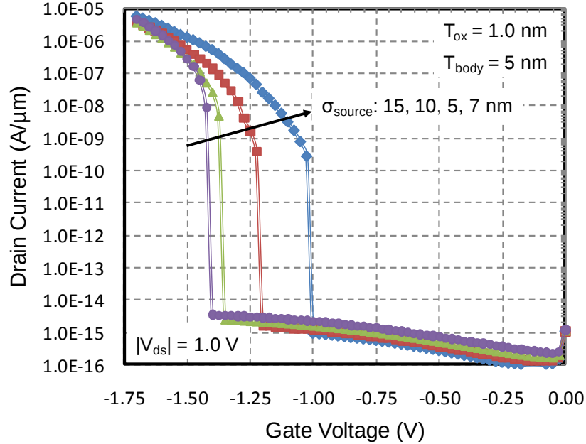
Figure 5.3: Simulation of UTB gTFET for fixed body thickness of 5 nm with varying lateral source profile abruptness. For less abrupt profile the overlap voltage V_{\text{ov}} is increased and turn on characteristic improves.
