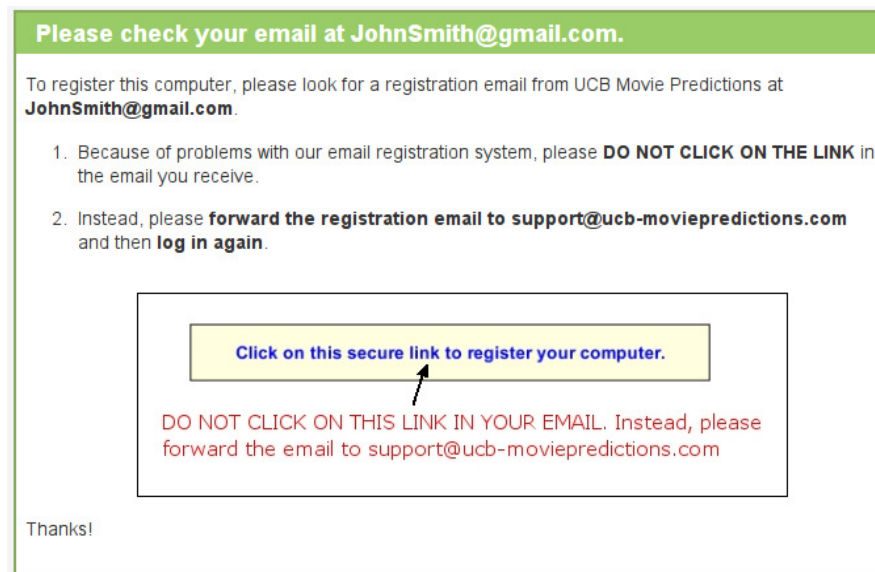
(a) Screenshot of the forwarding attack against email registration.
